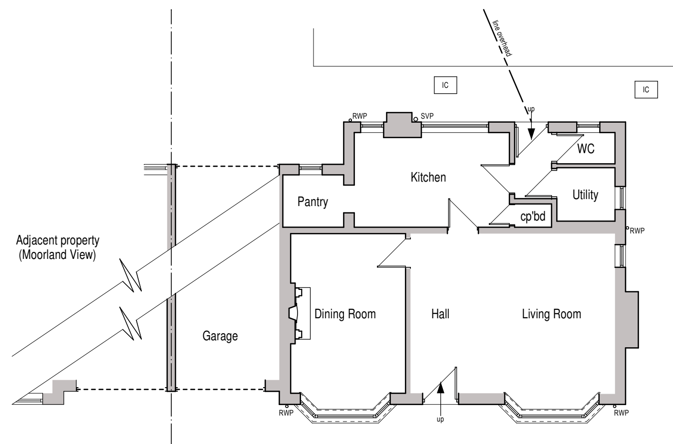
Part Ground Floor Plan
