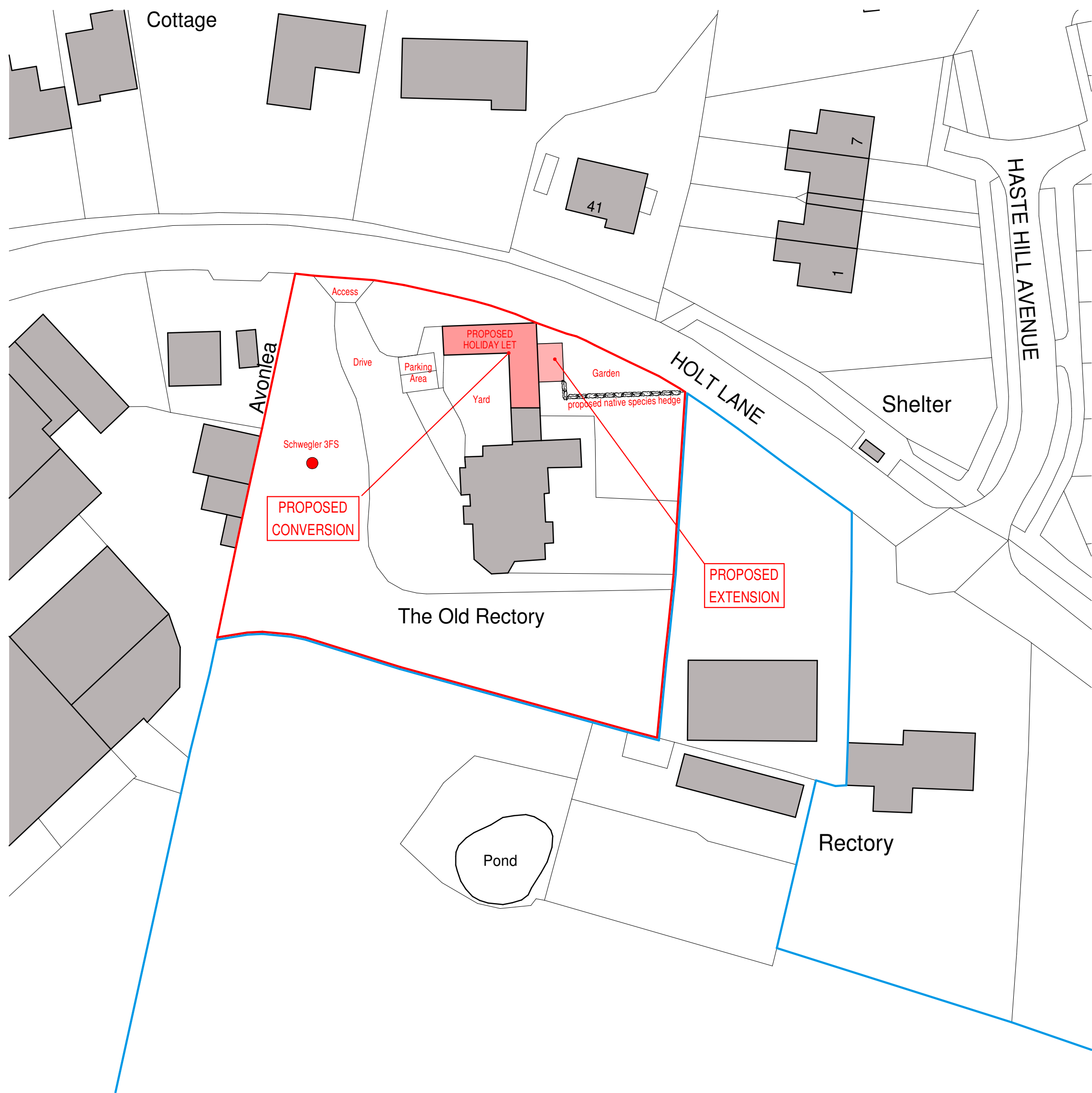
BLOCK PLAN
