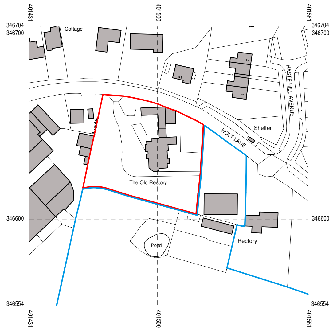
LOCATION PLAN
