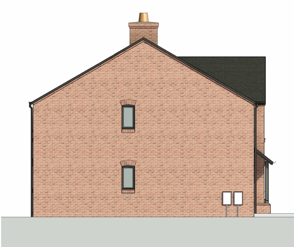
West Elevation 1 : 100
