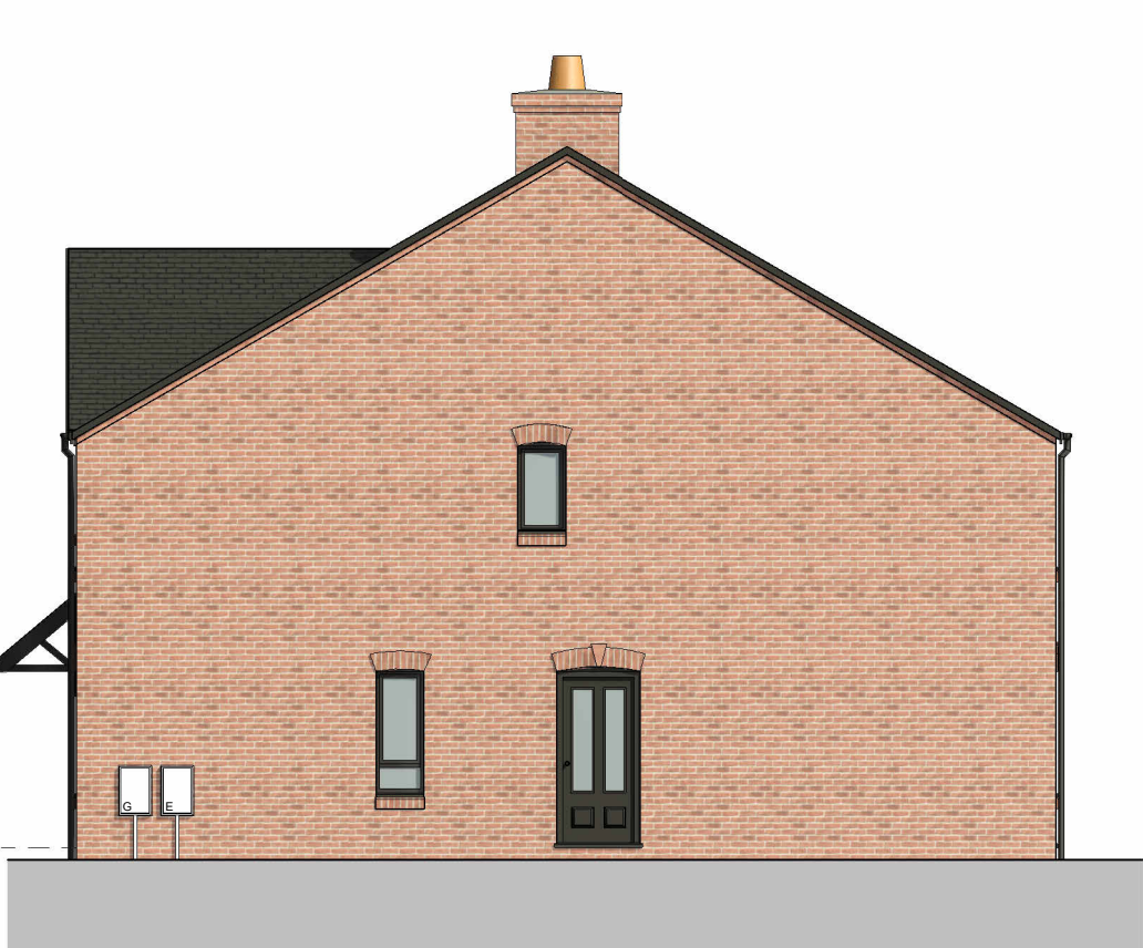
East Elevation 1 : 100
