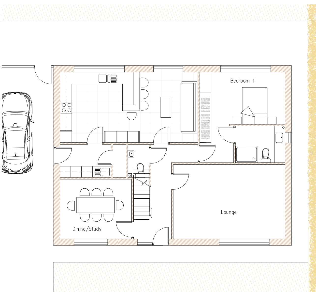
Ground Floor Scale 1:100
