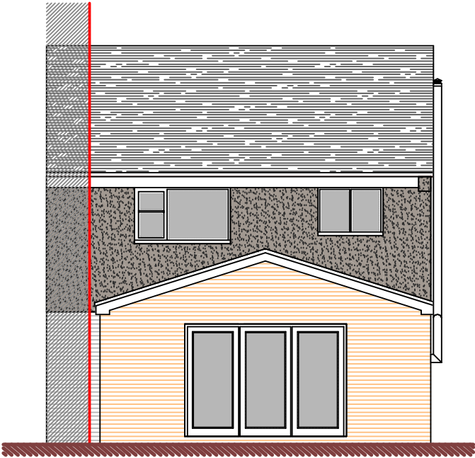
Rear Elevation
