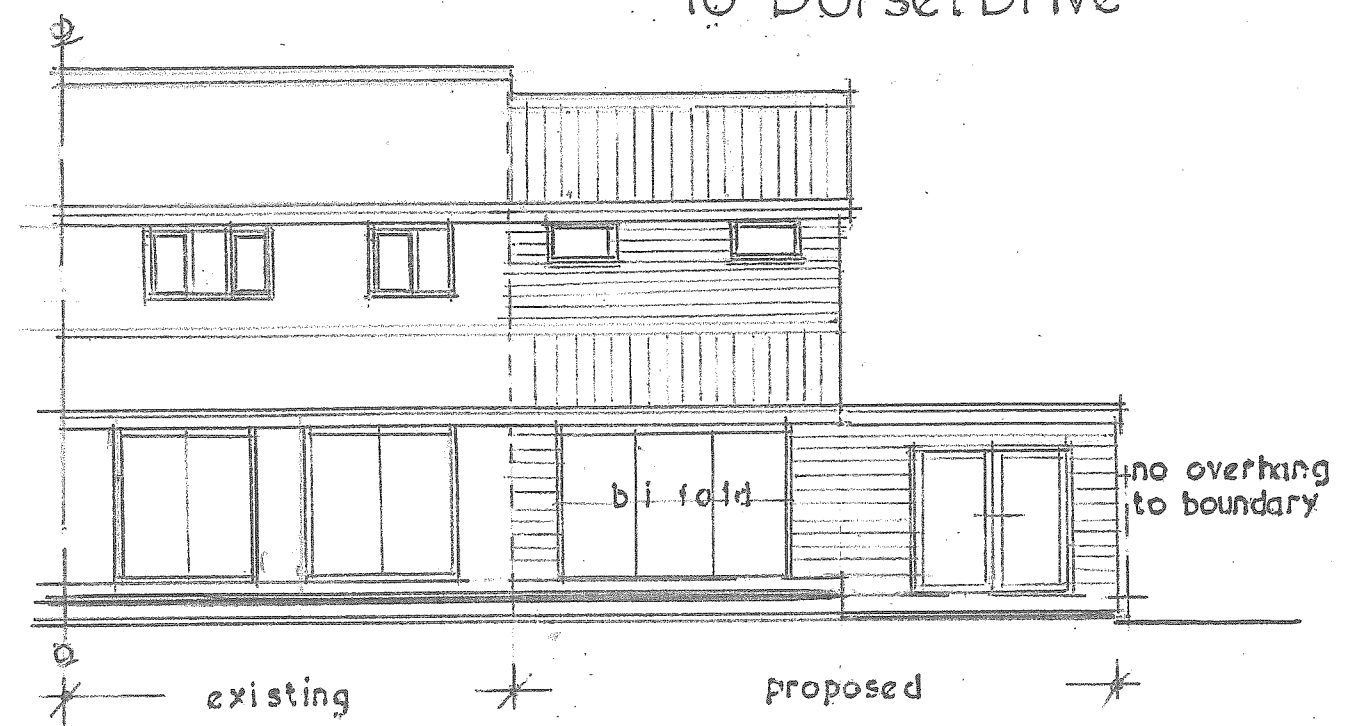
REAR ELEVATION AS PROPOSED to Garden. scale 1:100
