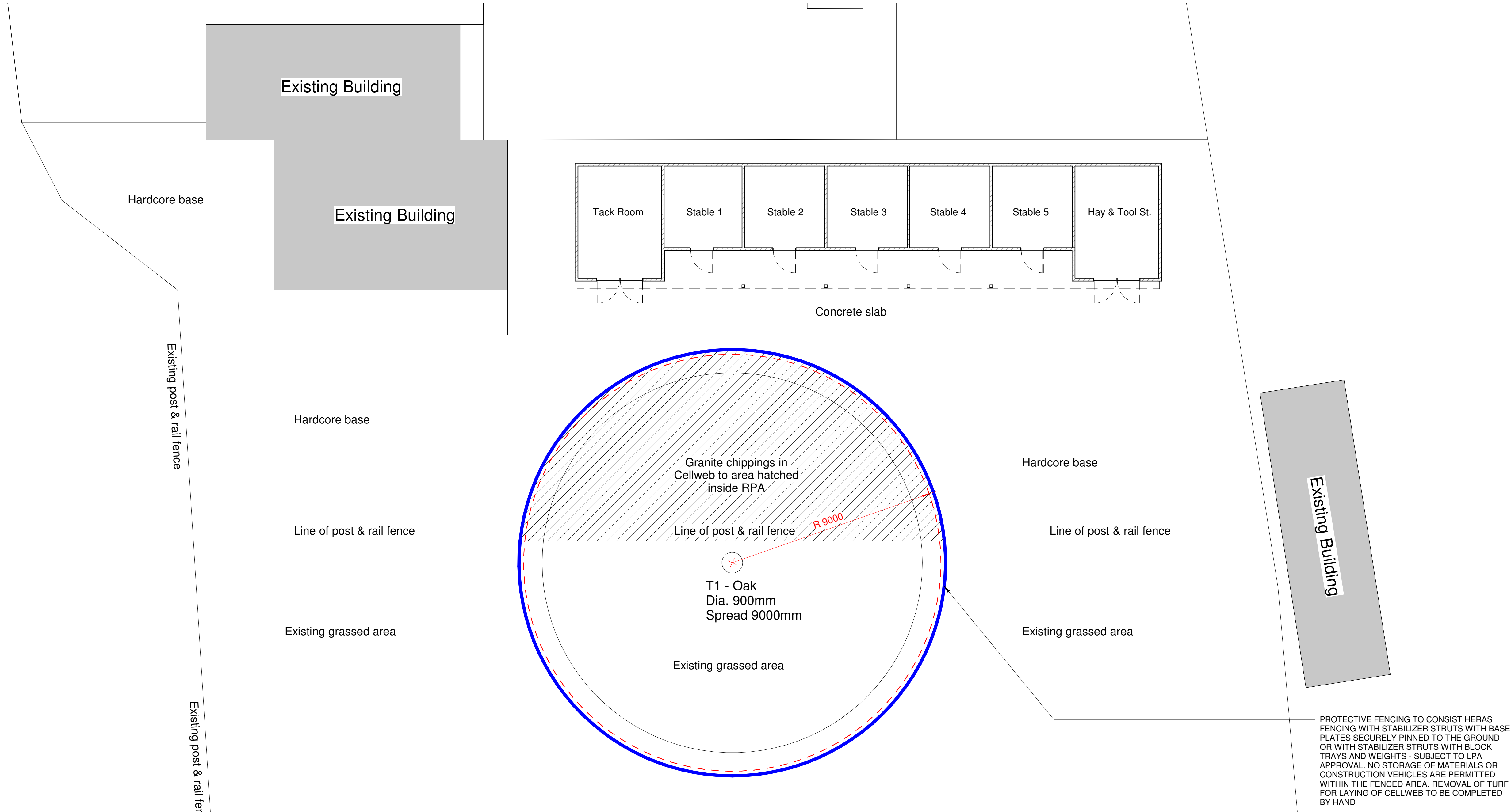
1 Proposed Part Block Plan 1 : 100
