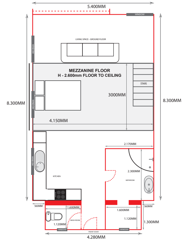
PROPOSED MEZZANINE LAYOUT
