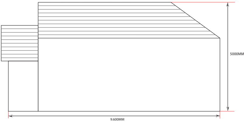
EXISTING ELEVATIONS SIDE VIEW
