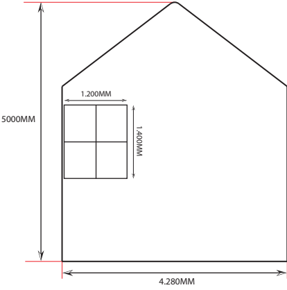
EXISTING ELEVATIONS REAR VIEW
