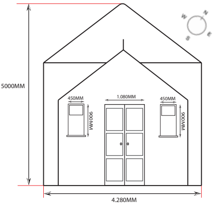
EXISTING ELEVATIONS REAR VIEW
