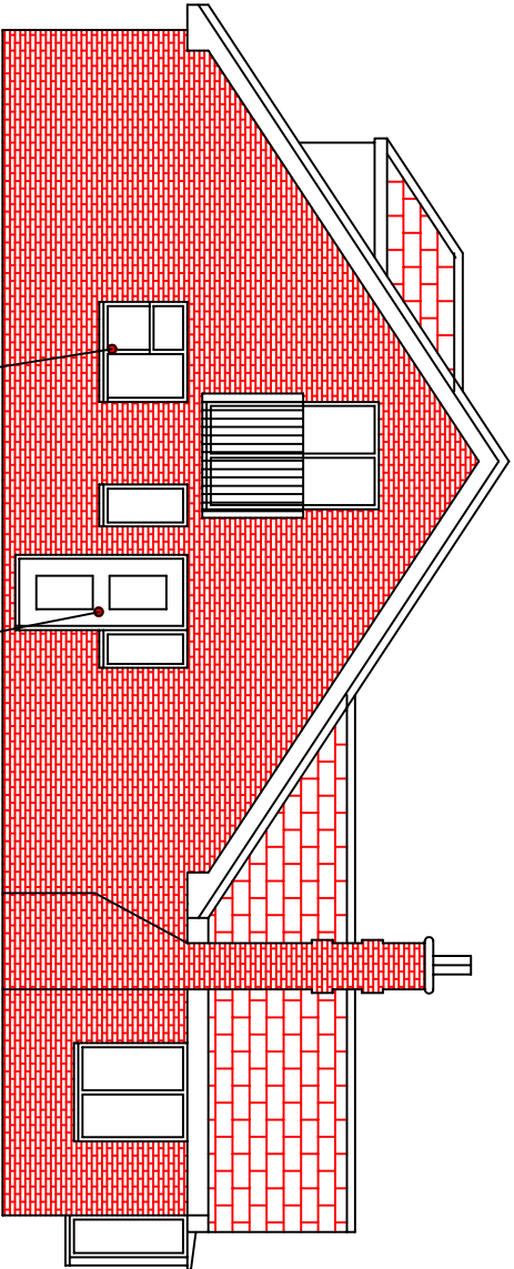
Left elevation (South West)
