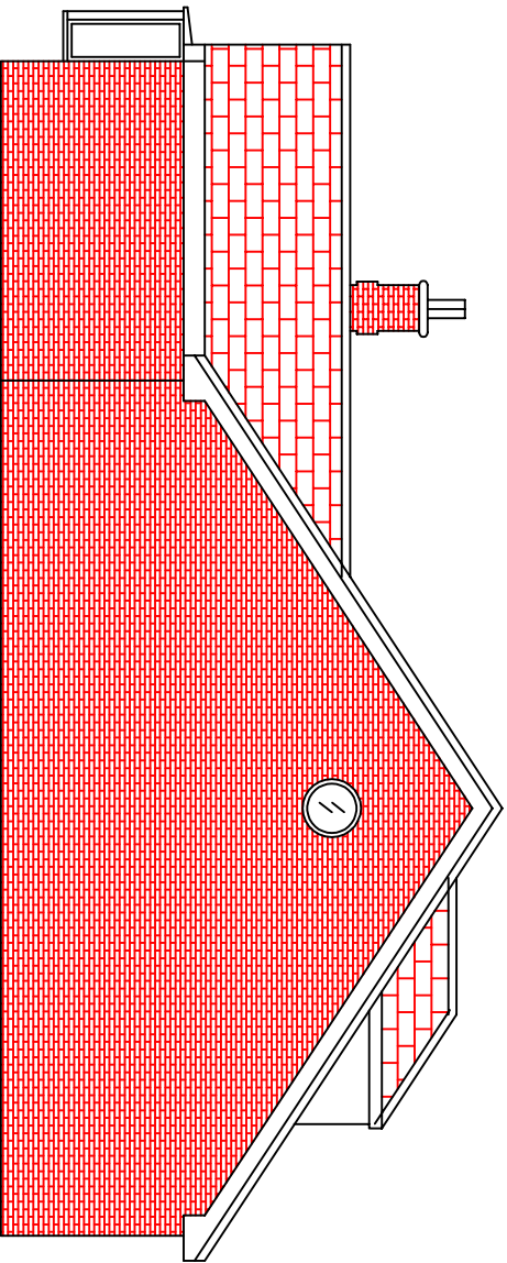
Right elevation (North East)
