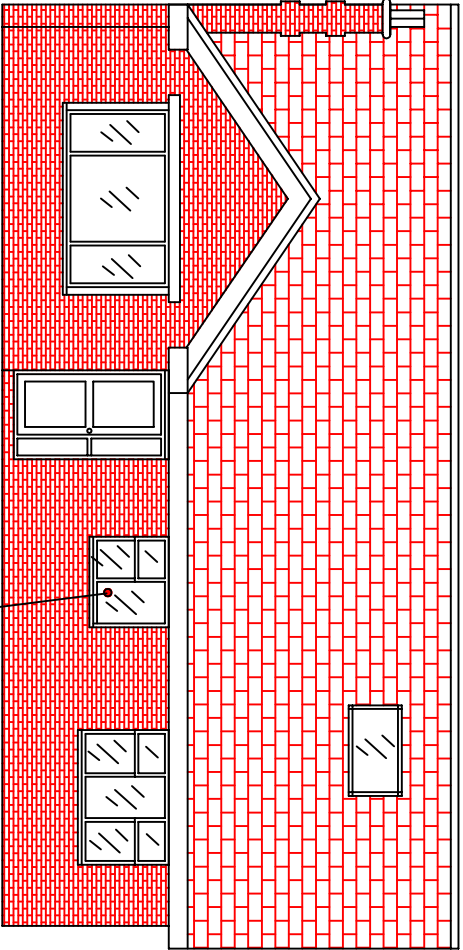
Front elevation (South East)
