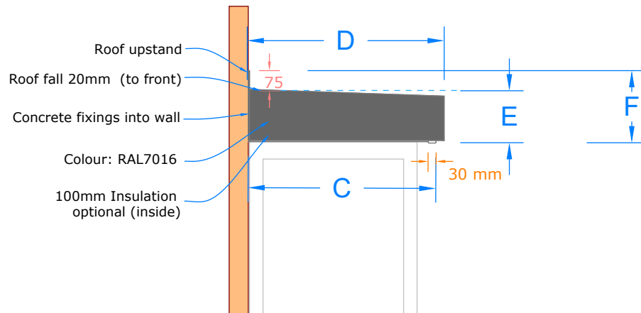
Side Elevation
