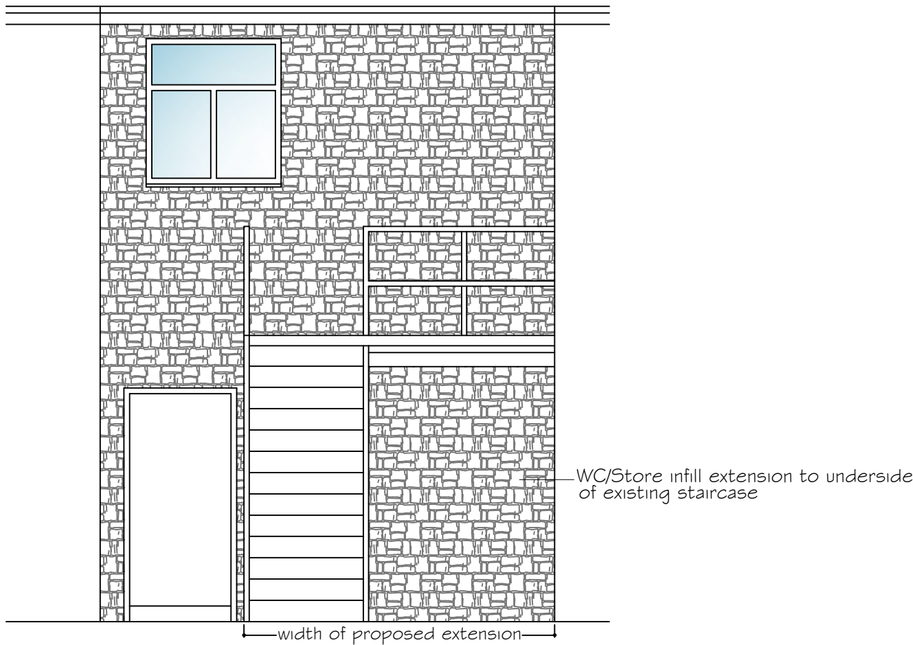
Proposed East Elevation (Rear)- 1:50
