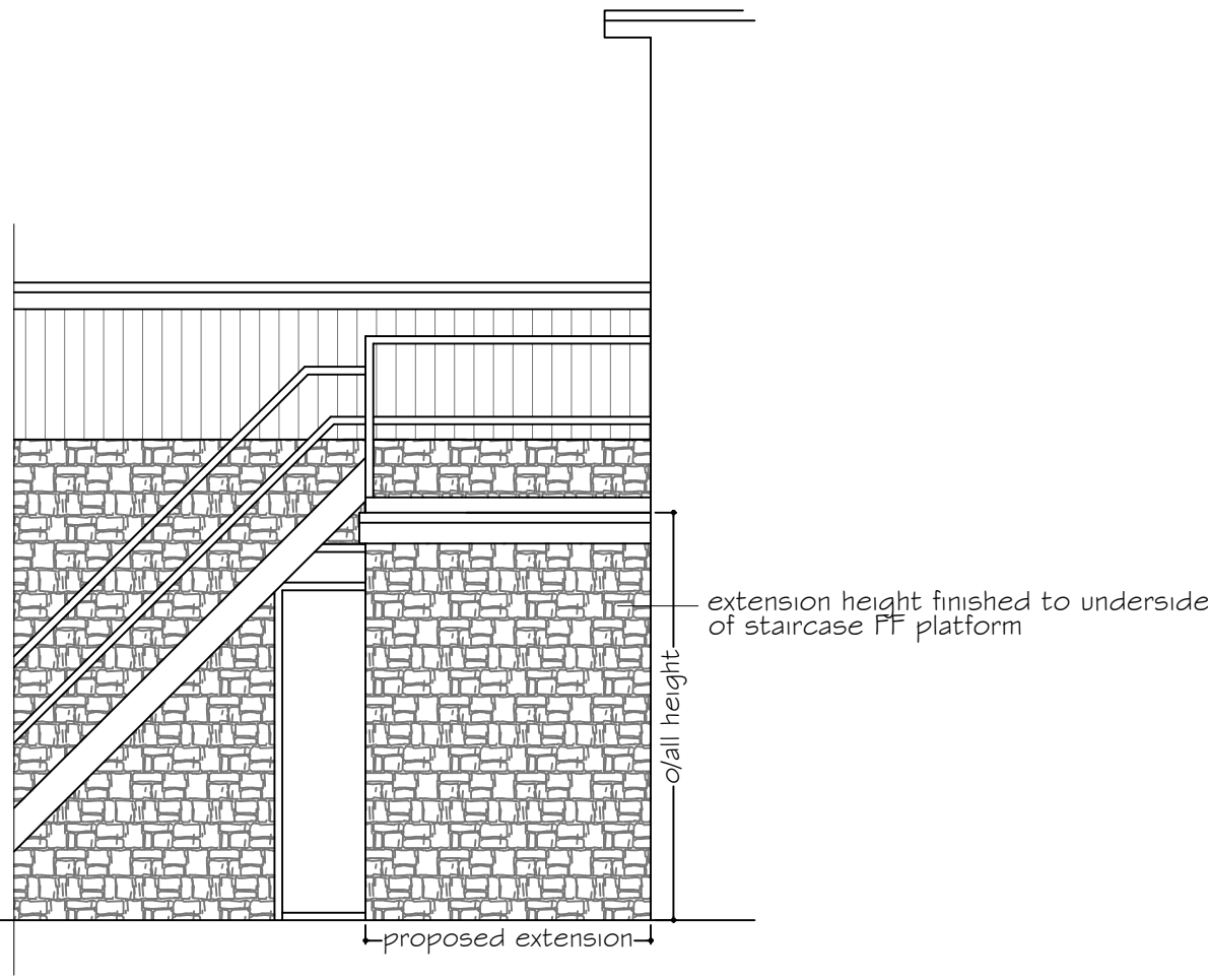
Proposed North Elevation (Side)- 1:50
