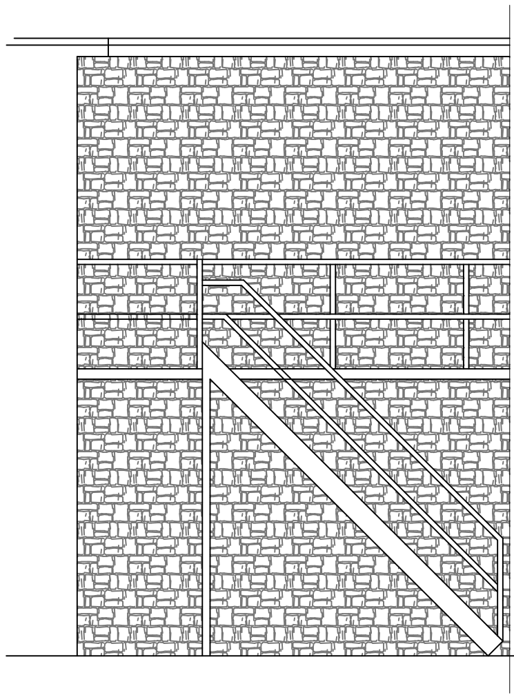
Existing South Elevation (Side)- 1:50
