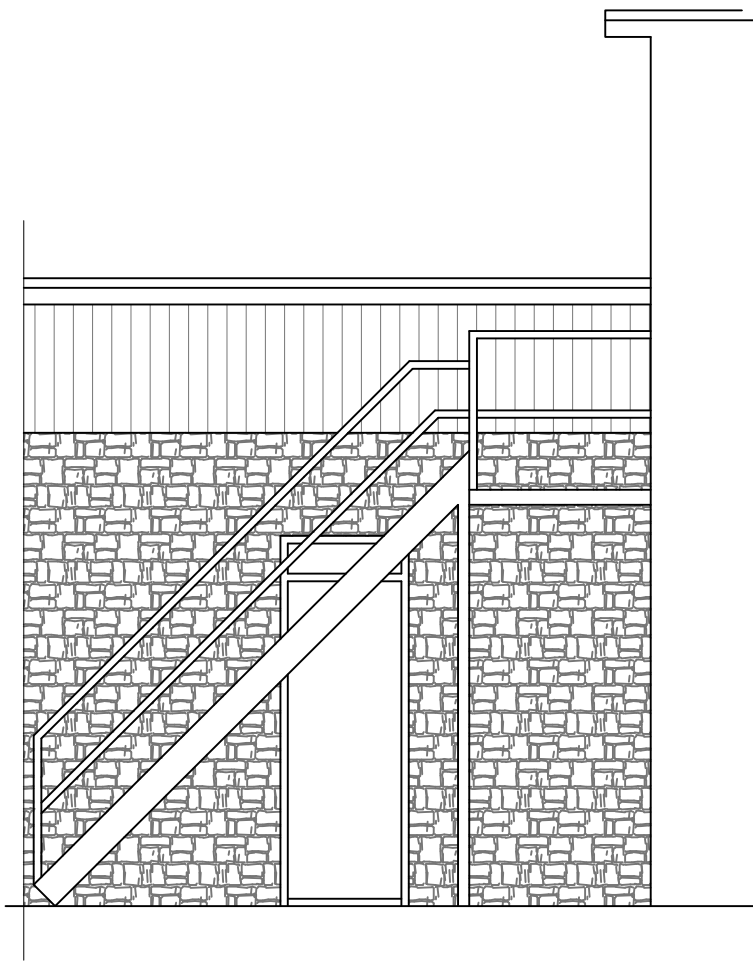
Existing North Elevation (Side)- 1:50
