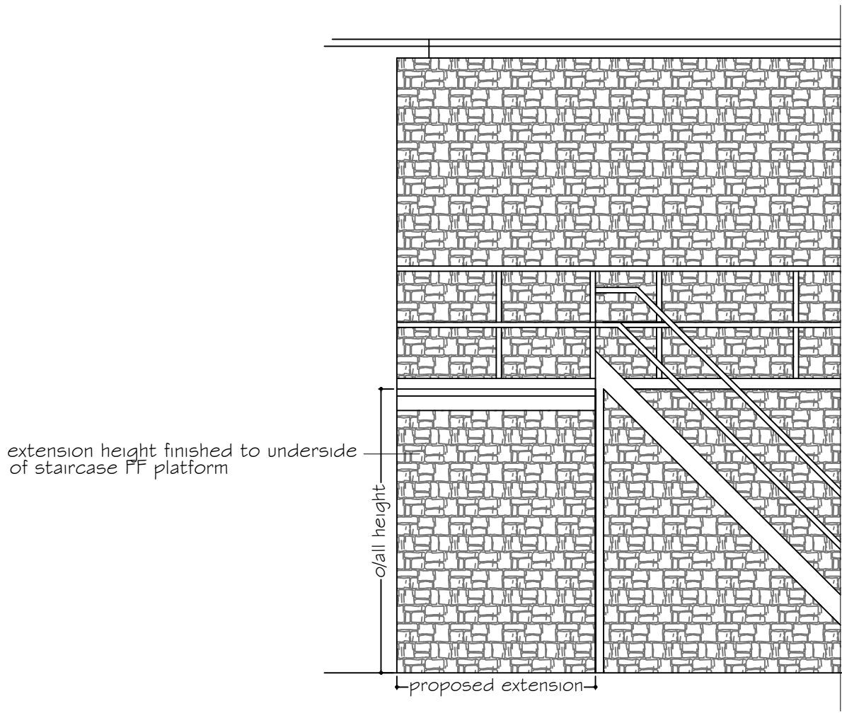
Proposed South Elevation (Side)- 1:50
