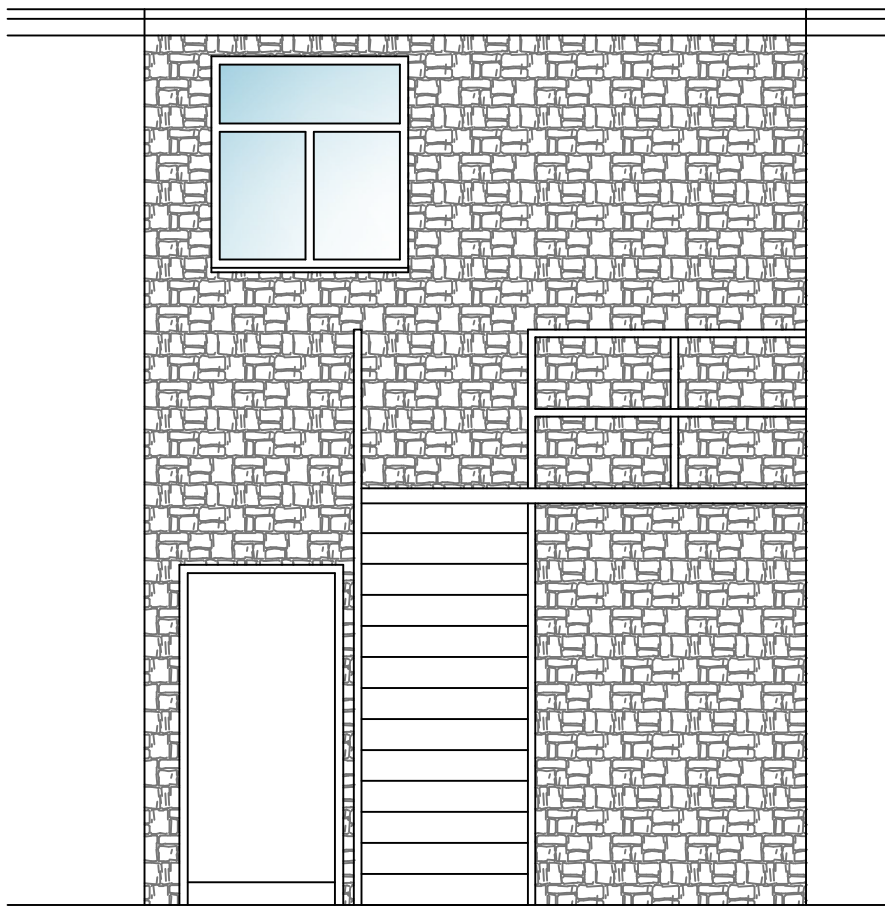
Existing East Elevation (Rear)- 1:50
