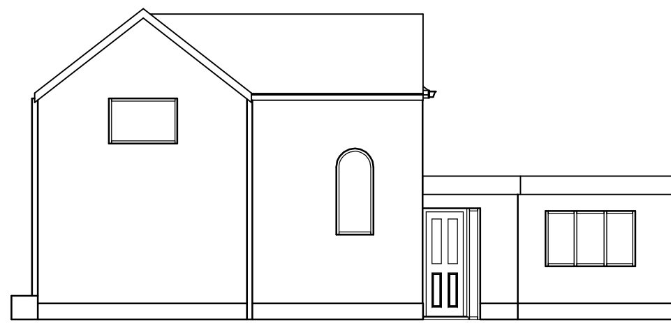
East Elevation
