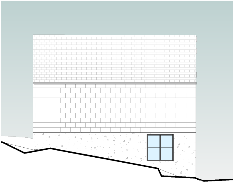
Side Elevation 1 : 100
