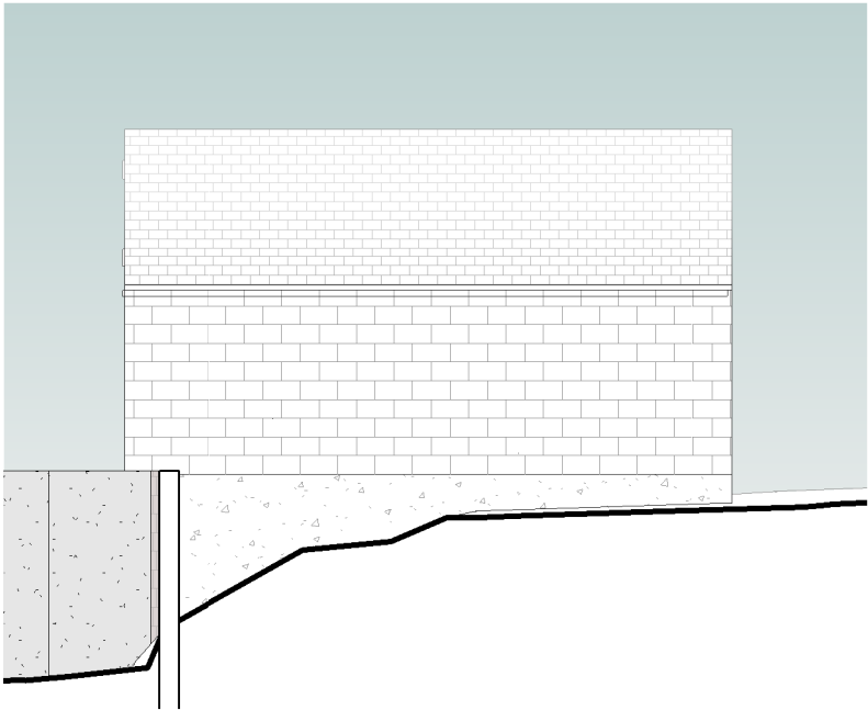
Side Elevation 1 : 100
