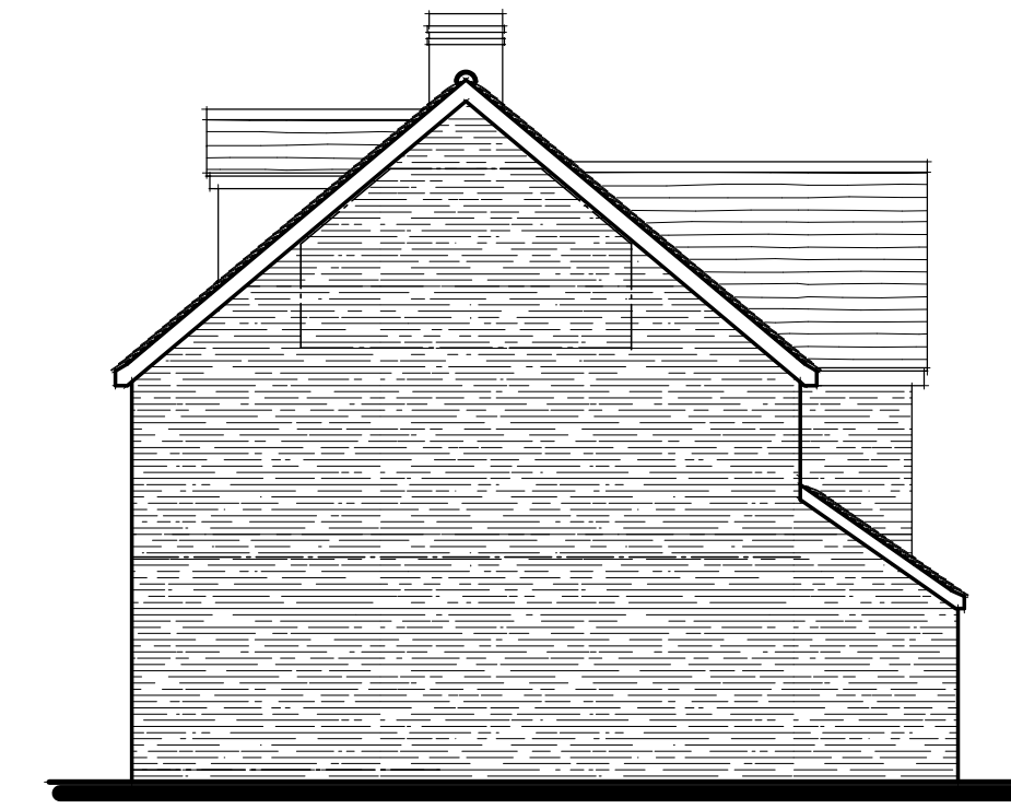
North Elevation
