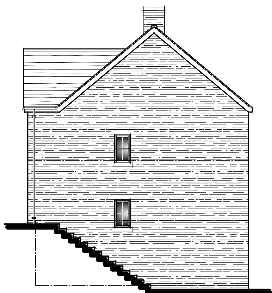
West Elevation
