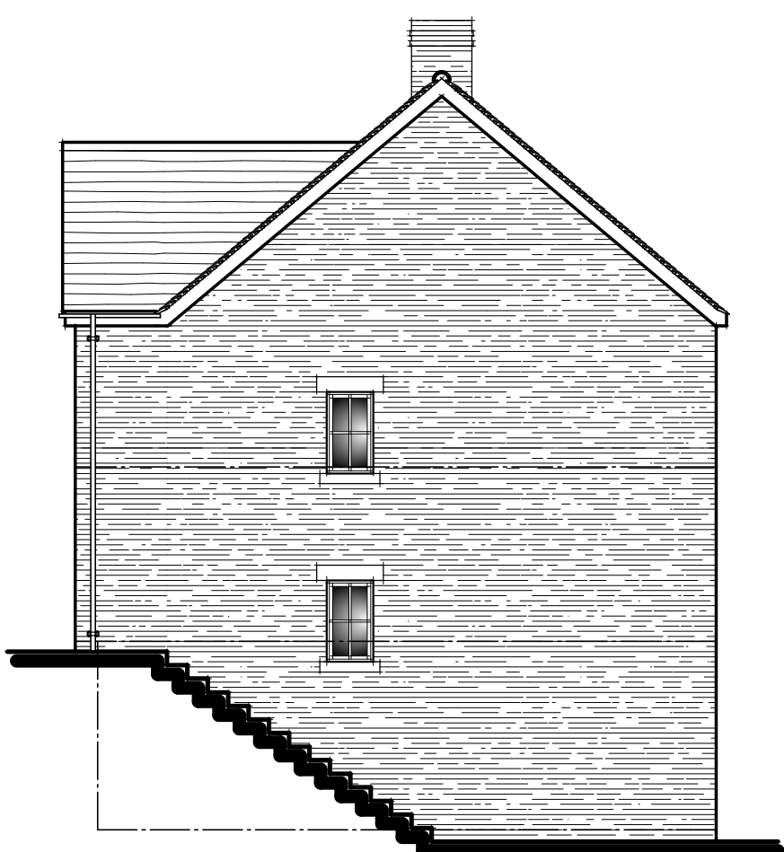
North Elevation
