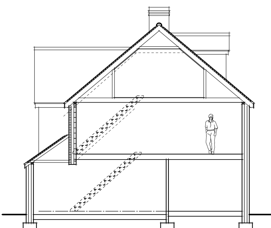
Section
