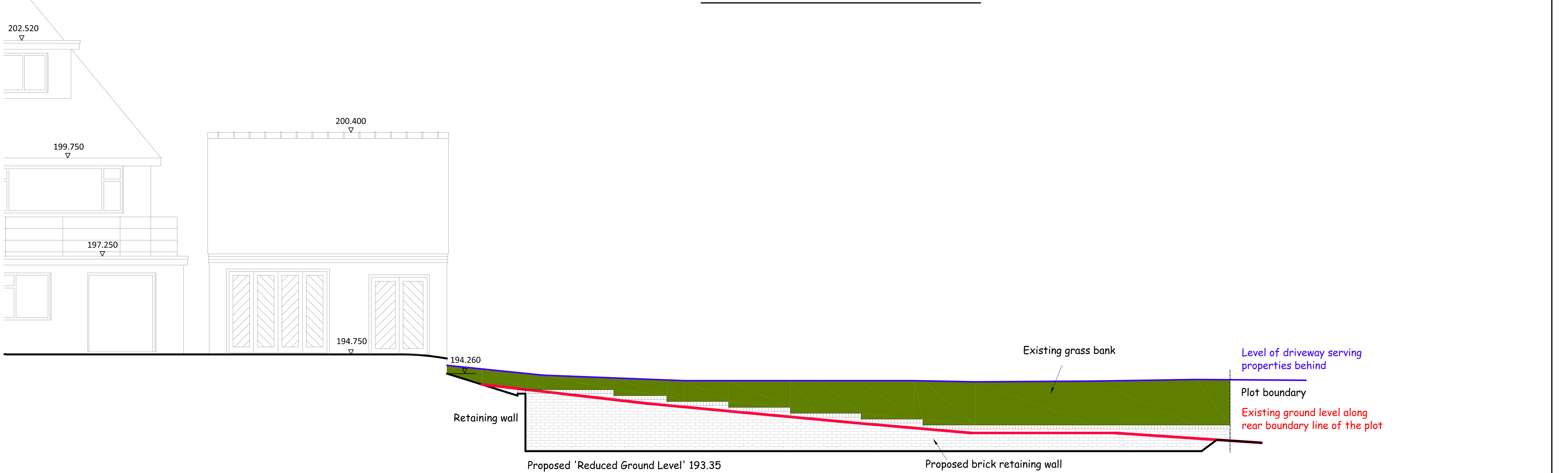
RETAINING WALL ALONG SOUTHWEST PLOT BOUNDARY
