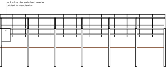
Rear Elevation
