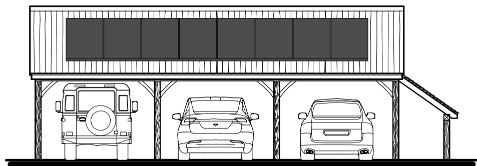
South Elevation
