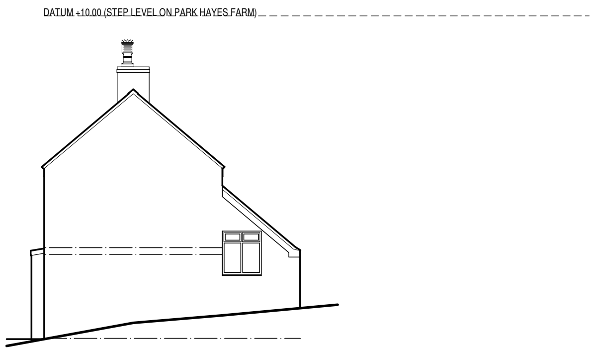
North Elevation
