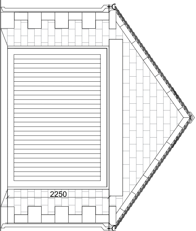
North West Elevation 1:50 @ A2
