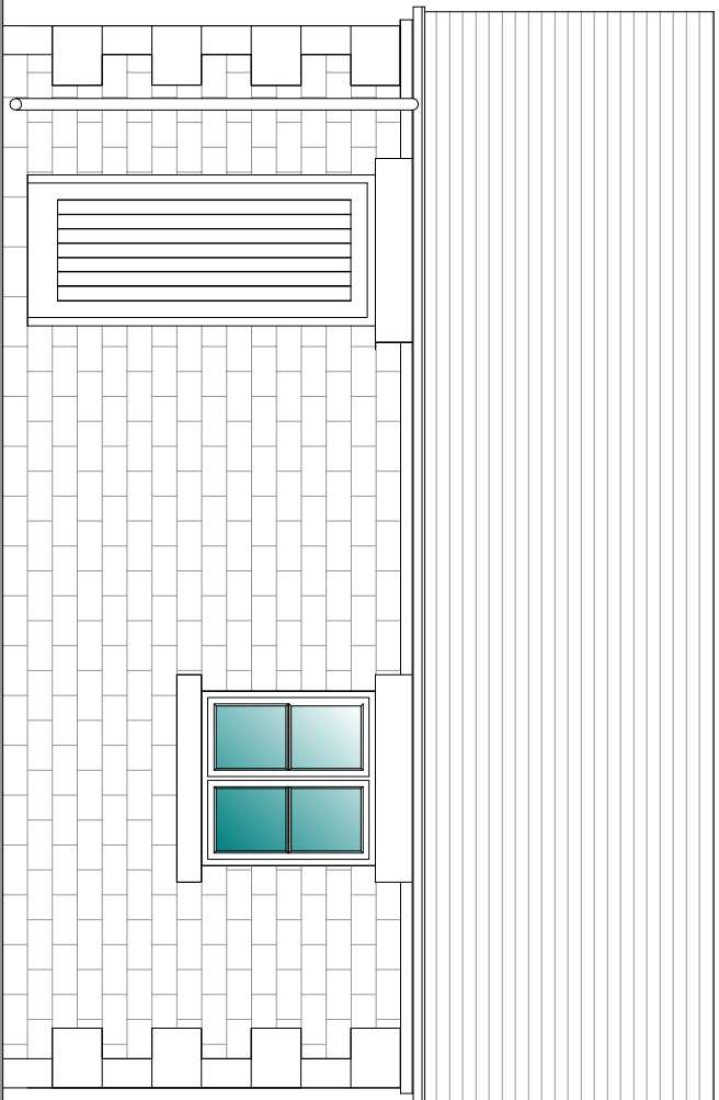
South West Elevation 1:50 @ A2
