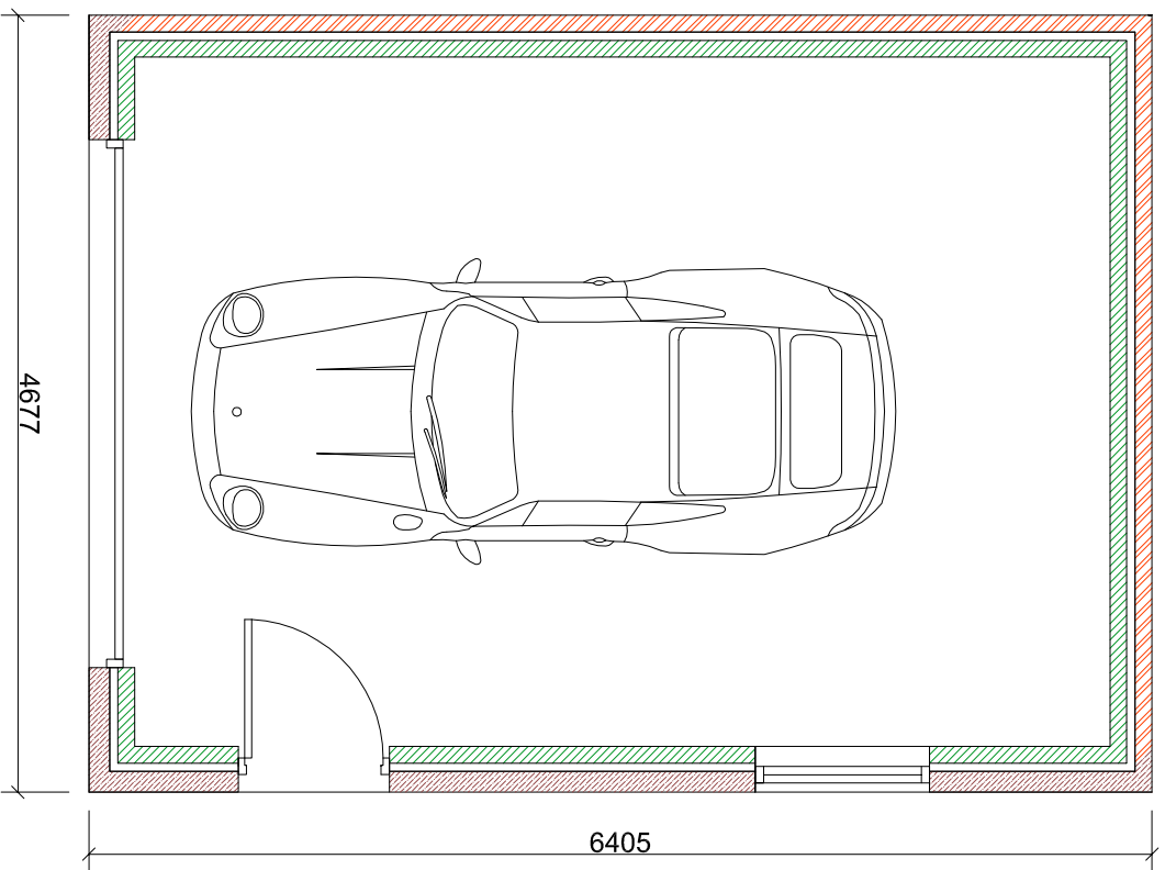
Floor Plan 1:50 @ A2
