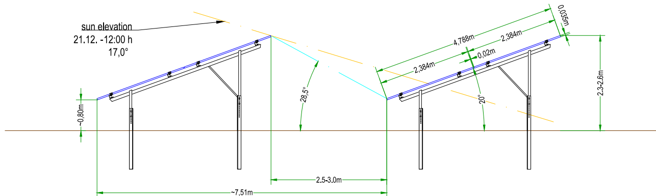
SIDE ELEVATION - 1:100
