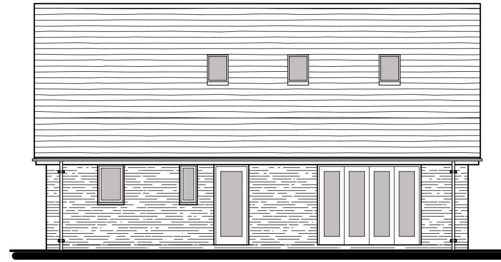
South Elevation
