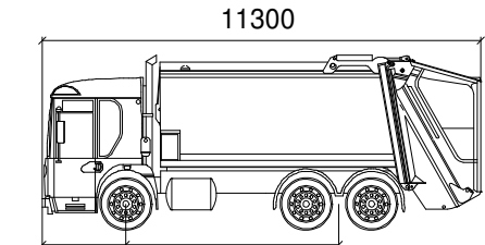
Dennis Eagle 6X4 RHS 2013 mm Width : 2500 Track : 2500 Lock to Lock Time : 6.0 Steering Angle : 32.1
