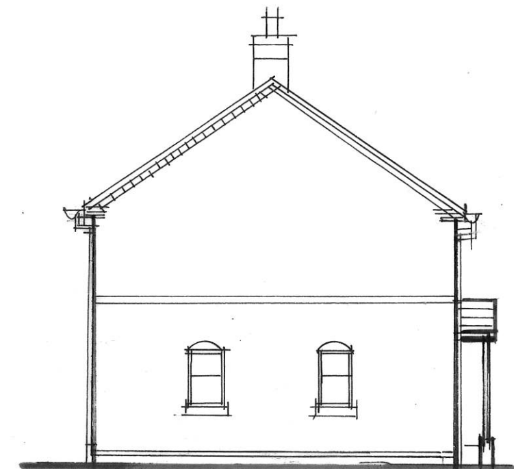
SIDE ELEVATION
