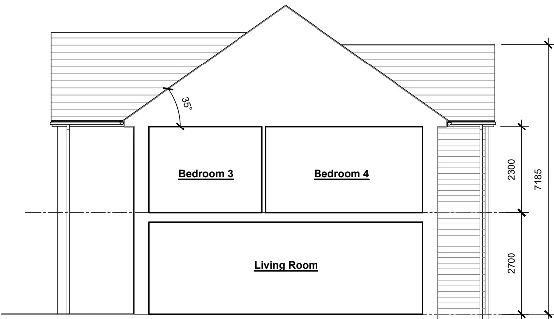
Section
