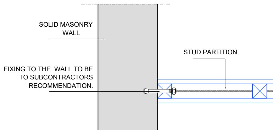
DETAIL 2 TYING-IN OF NEW STUD WALLS TO MASONRY WALLS SCALE 1/10
