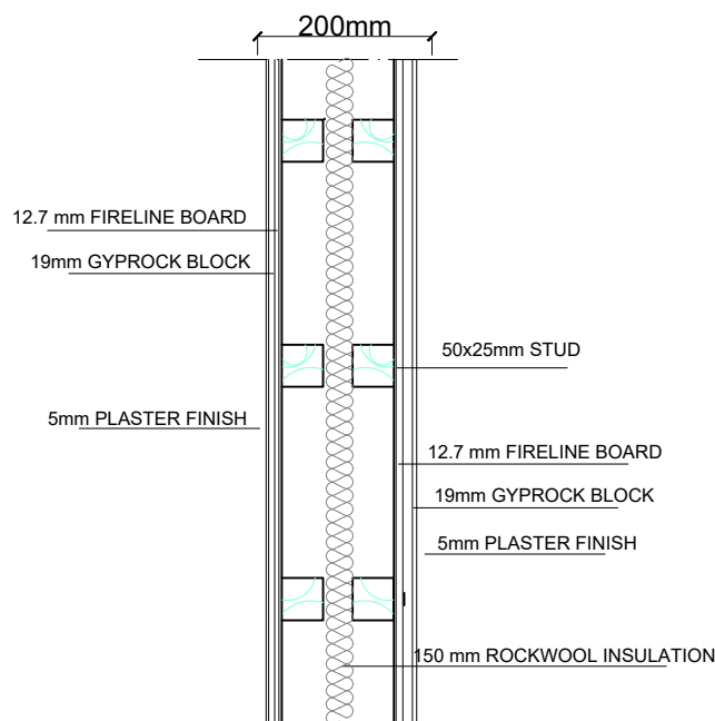
DETAIL 1 FIRE&SOUND&SMELL INSULATION DETAIL TO PARTITION WALL BETWEEN THE ACCOMMODATION AND THE COMMON STAIRCASE & INNER BEDROOMS
