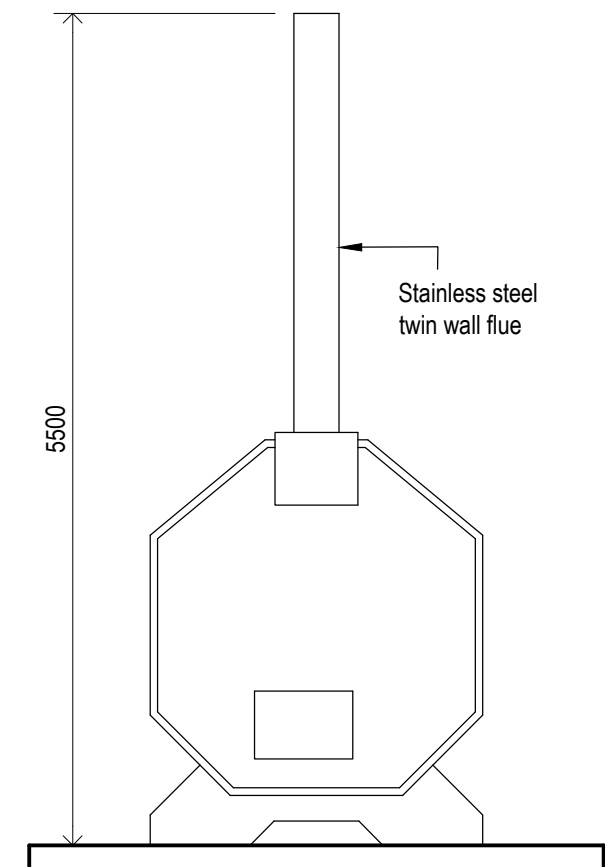
Rear Elevation
