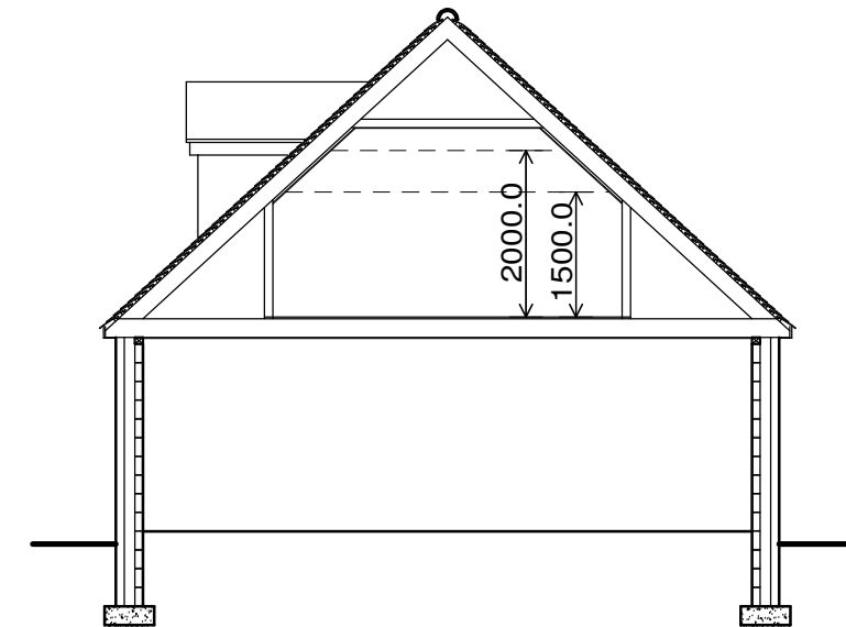
Section
