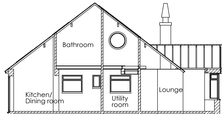
Proposed SECTION F-F
