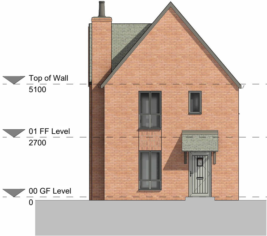
South Elevation 1 : 100
