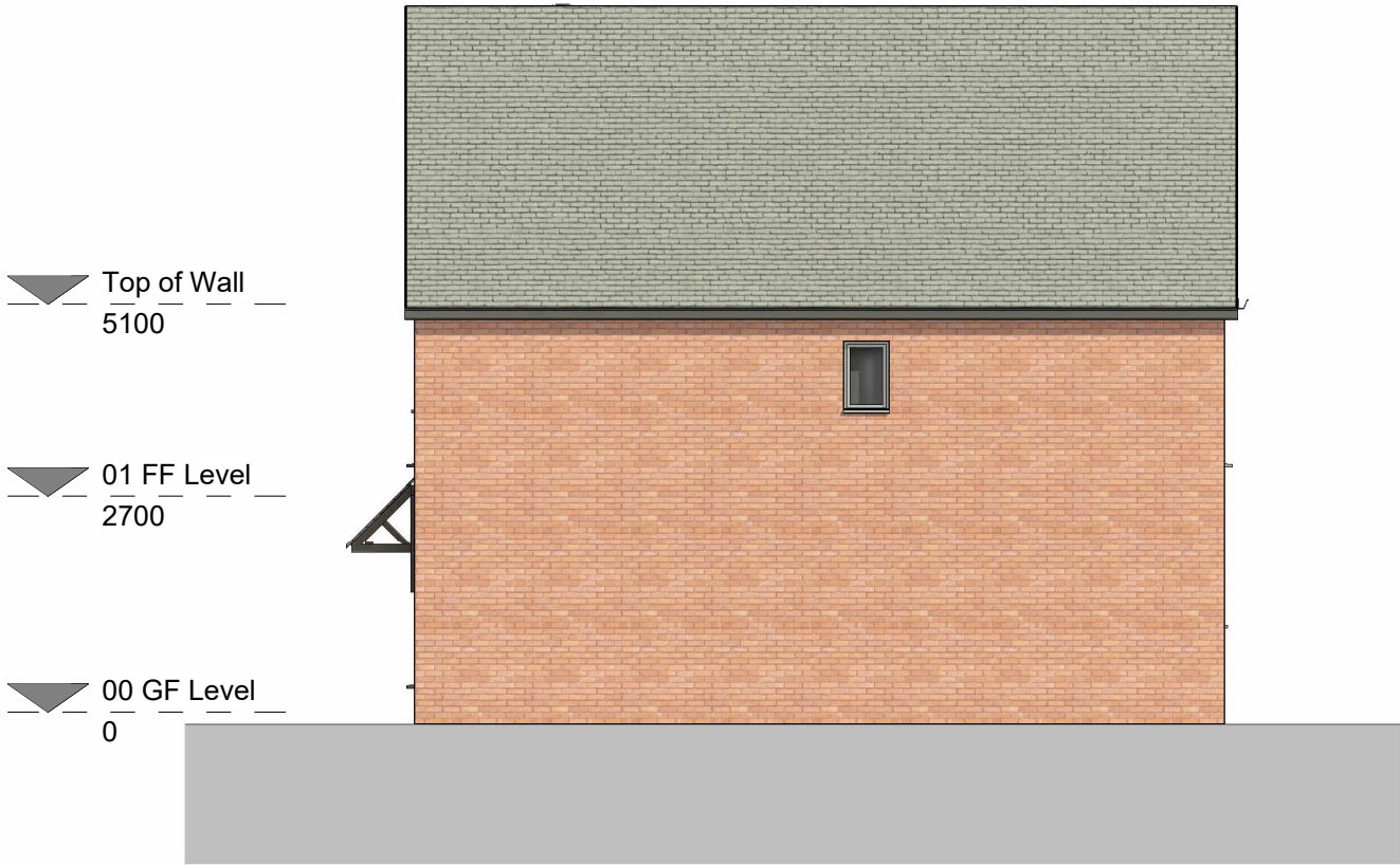
East Elevation 1 : 100
