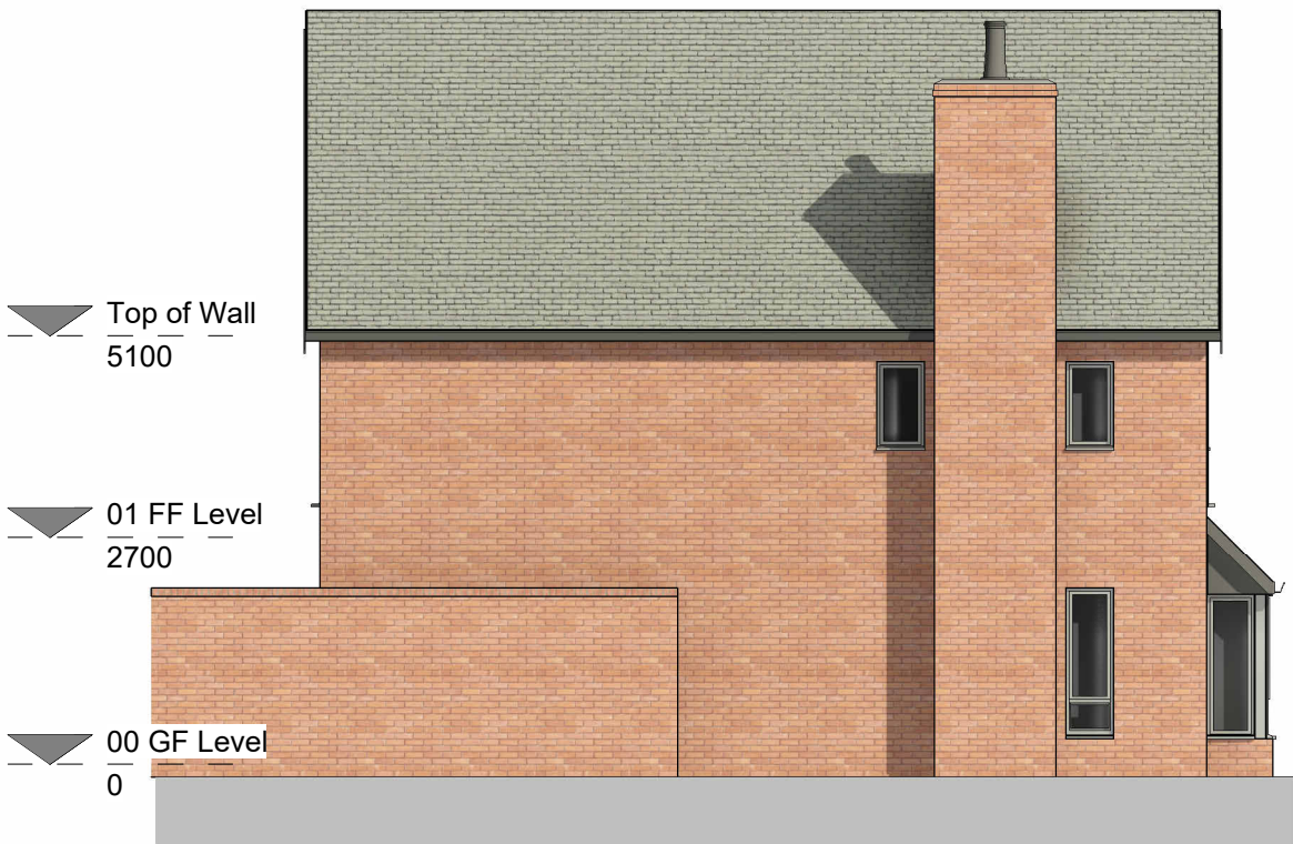
East Elevation 1 : 100
