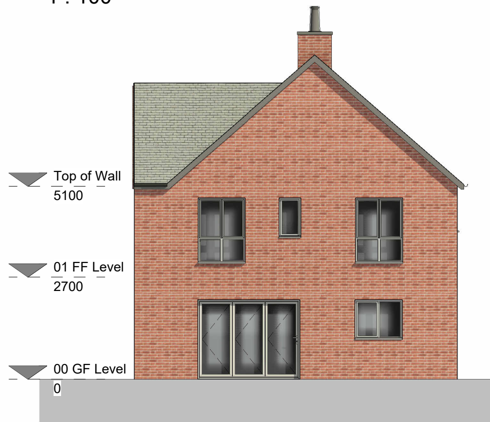
South Elevation 1 : 100
