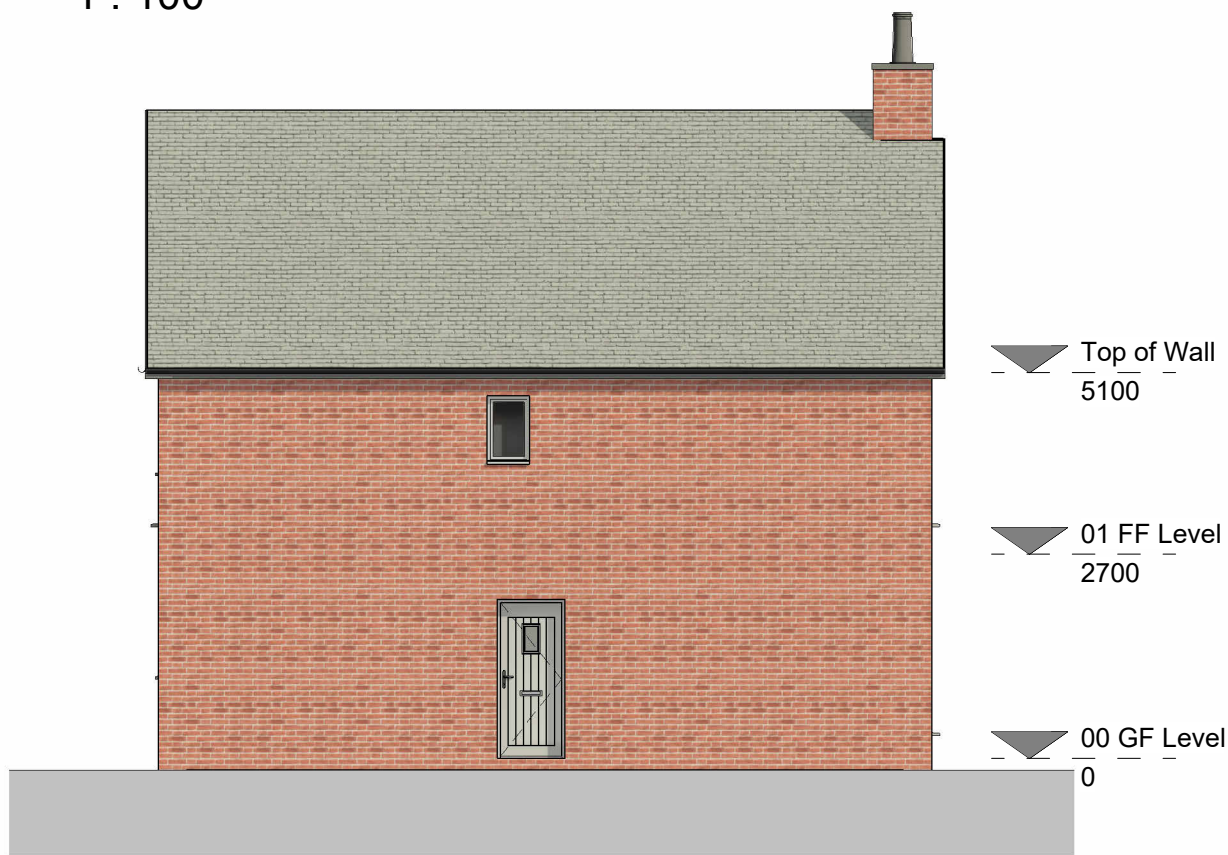
East Elevation 1 : 100
