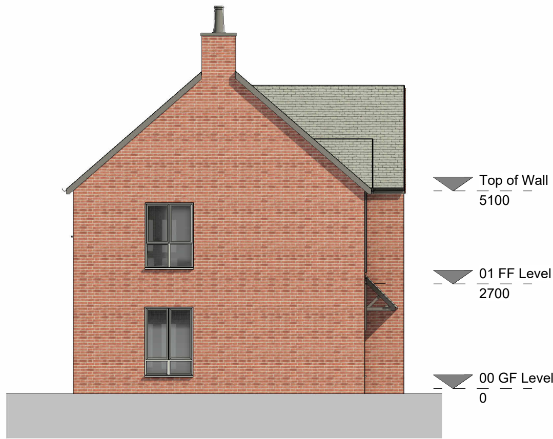
North Elevation 1 : 100
