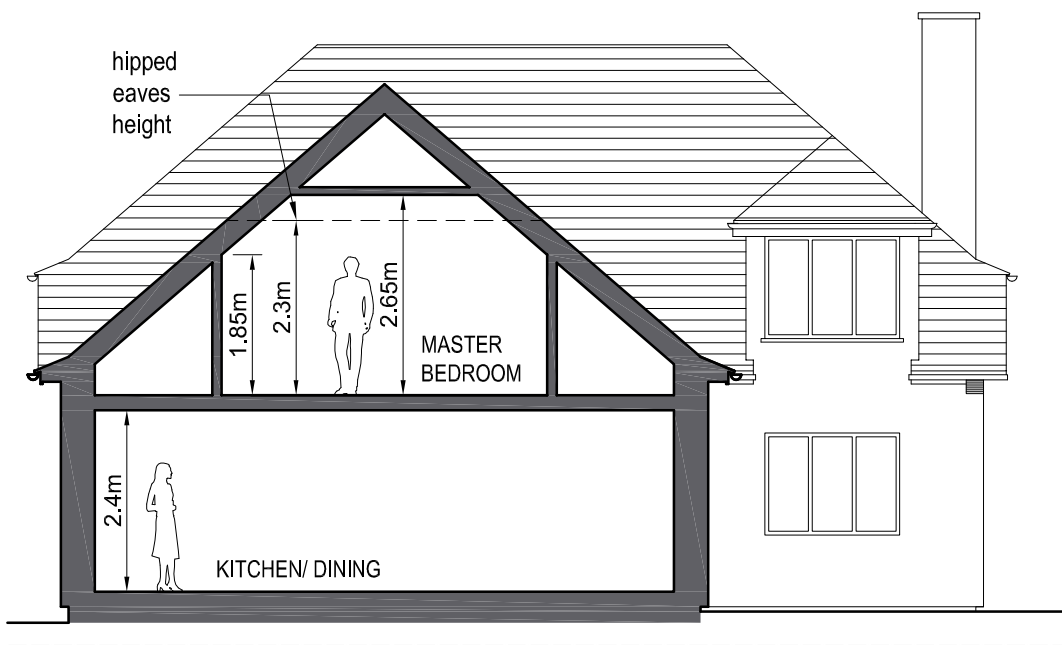
SECTION B-B
