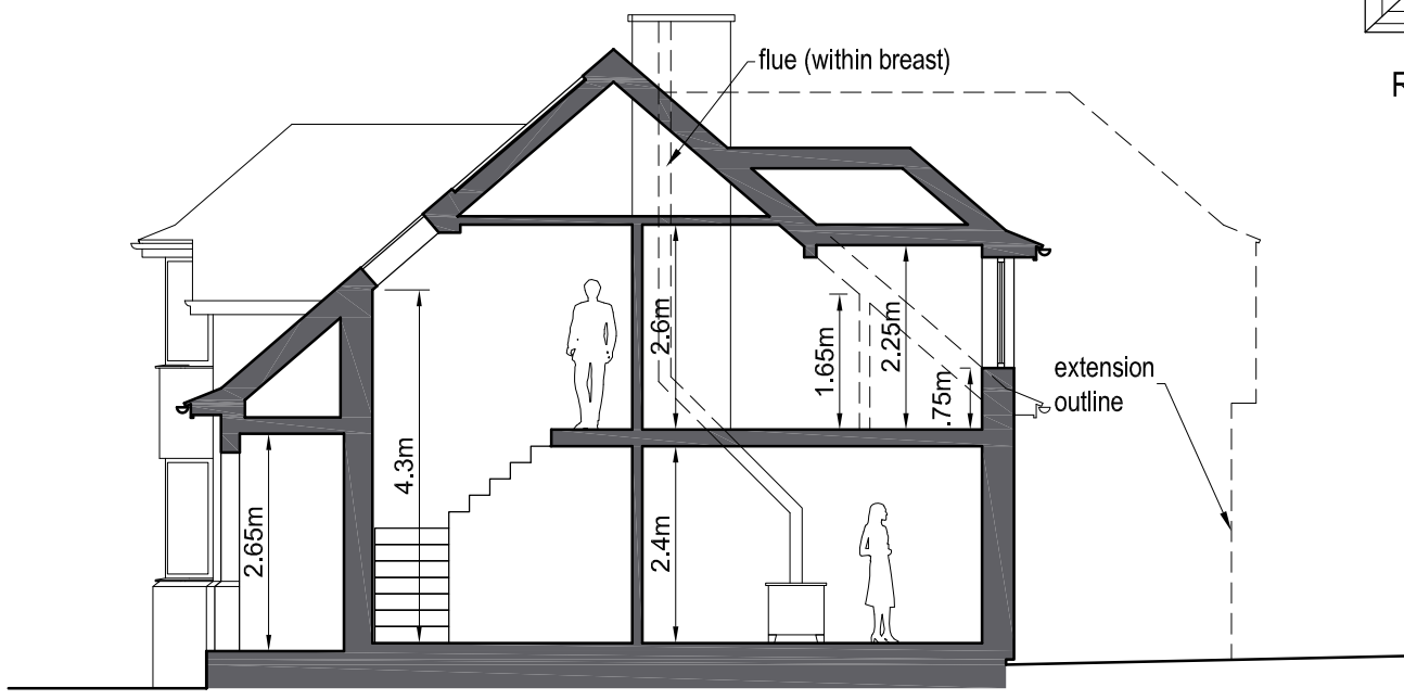
SECTION C-C
