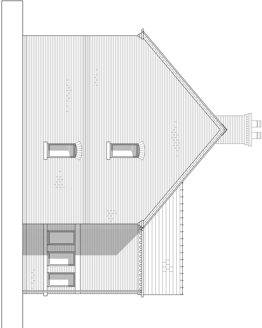
elevation D scale 1 / 100
