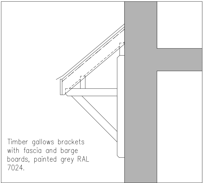
Entrance Canopy. (Plots 1–2–3) Scale 1:20
