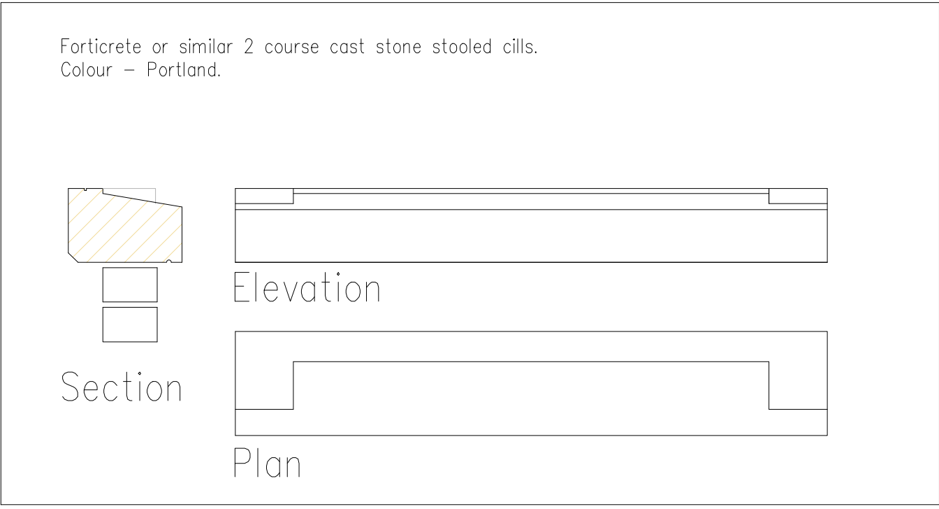
Window Cills (Plots 1–2–3) Scale 1:10
