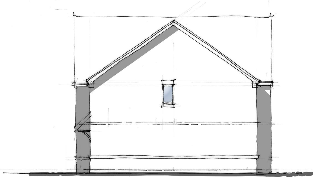
[House Type B] Proposed Side Elevation [House Type B] [Scale 1:100]
