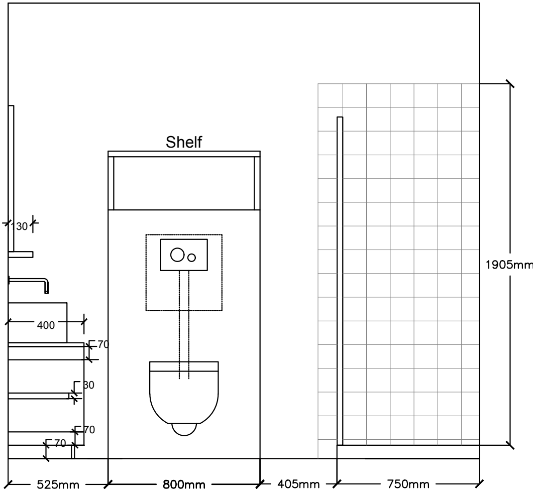
02 The Logshed Bathroom 2 - Elevation 1:20
