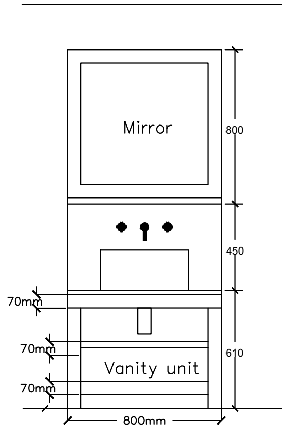
03 Typical Bathroom - Vanity Unit Elevation 1:20
