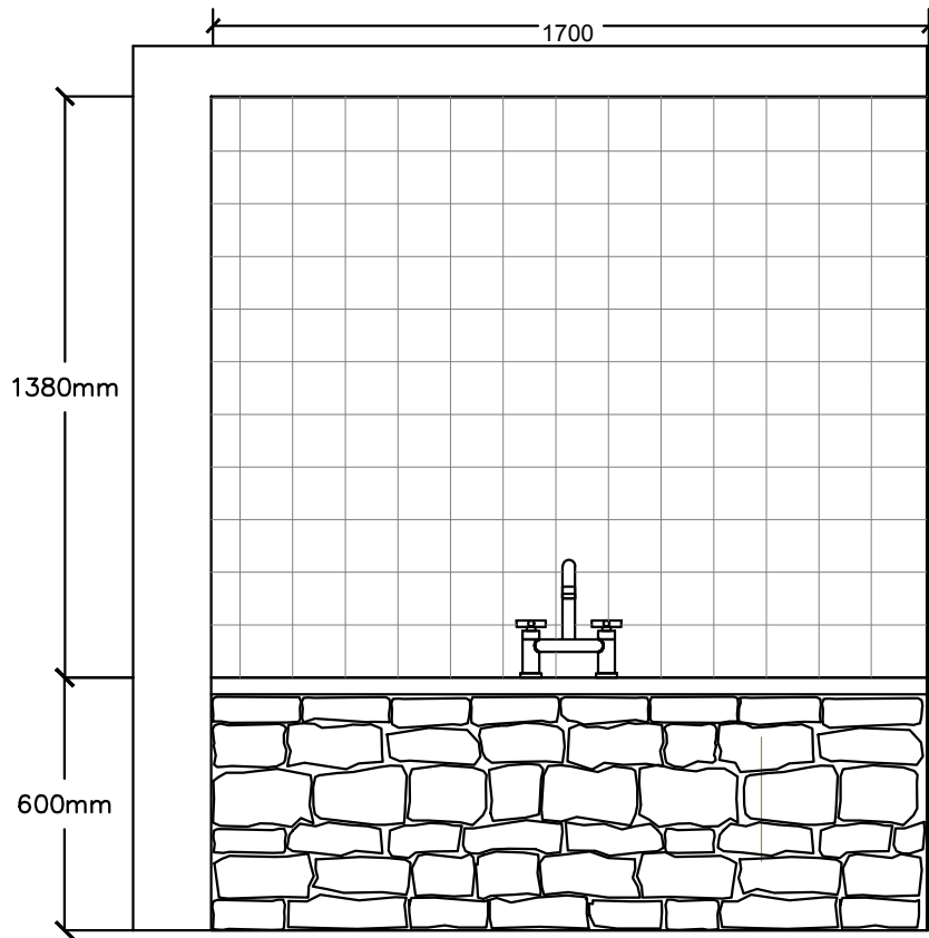
05 Typical Bathroom - Bath Elevation 1:20
