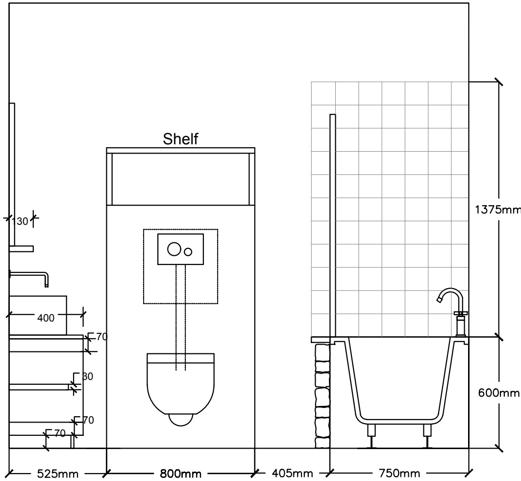
01 The Logshed Bathroom 1 - Elevation 1:20
