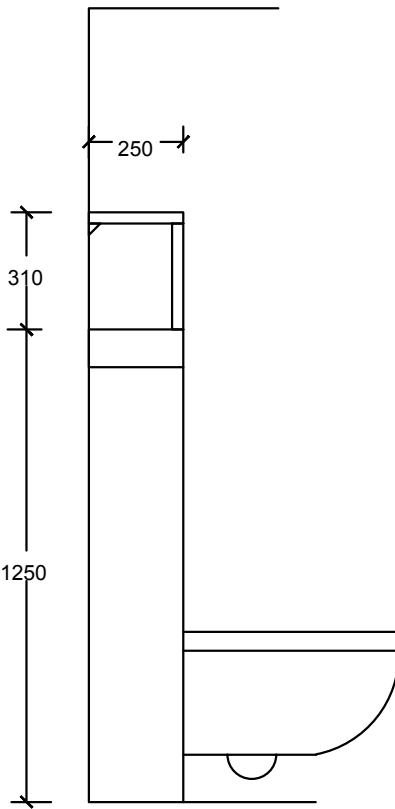
04 Typical Bathroom - WC Section 1:20
