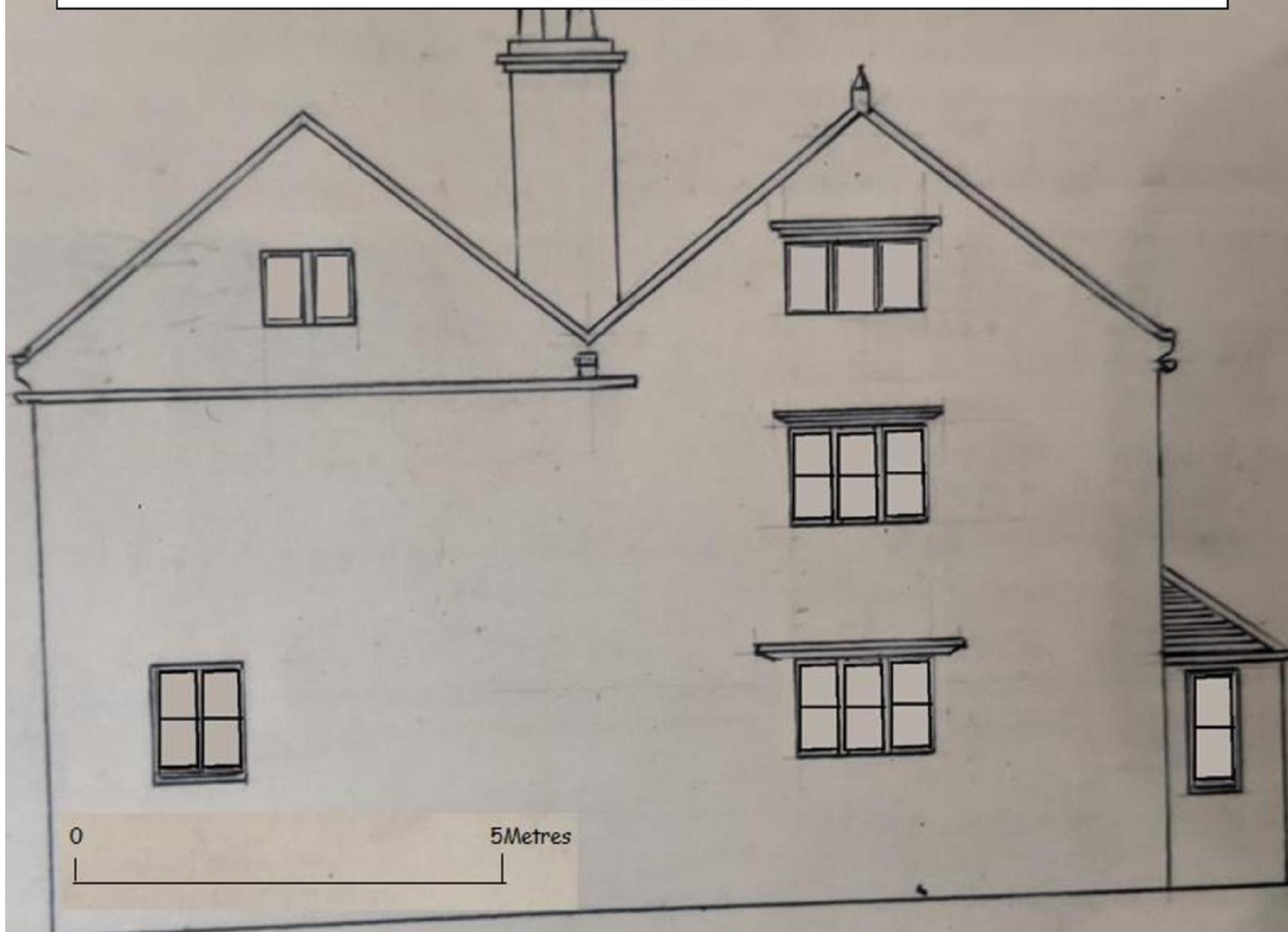
North West Elevation
