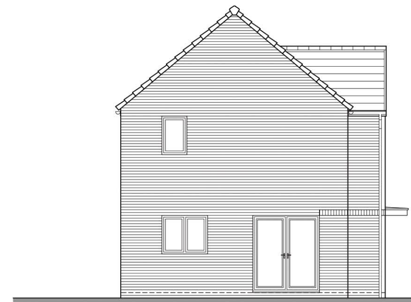
Side Elevation
