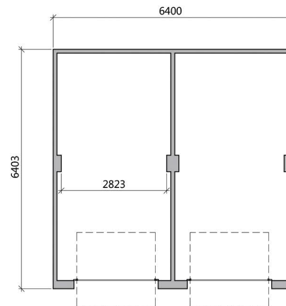
Floor Plan
