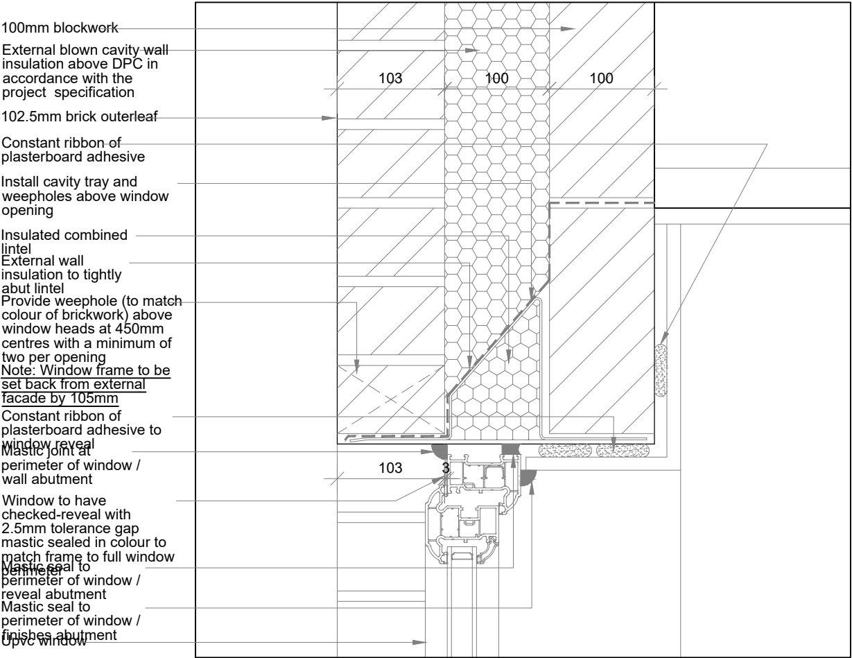
detail 01 - window head
