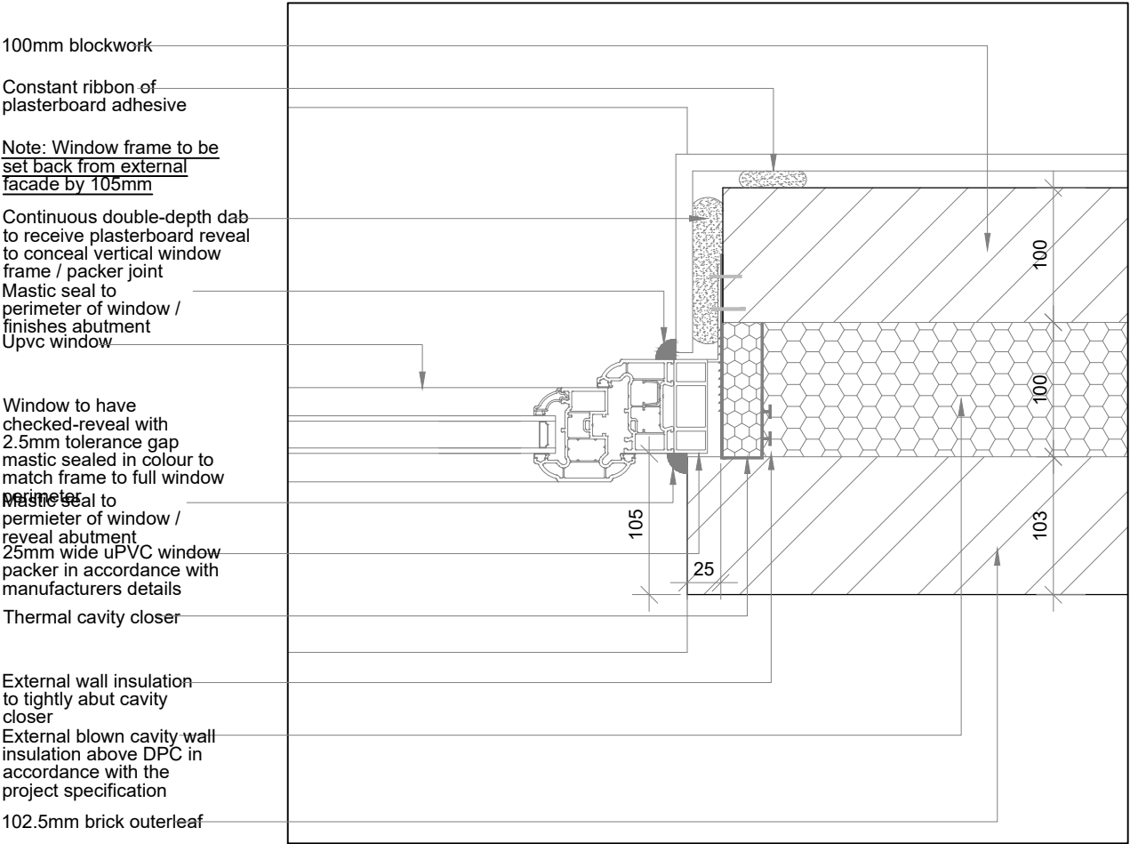
detail 02 - window jamb
