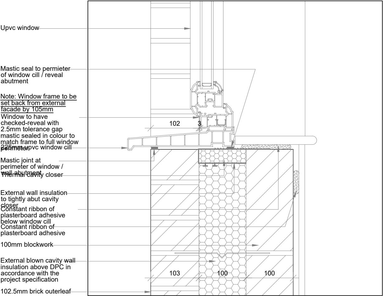
detail 03 - window cill
