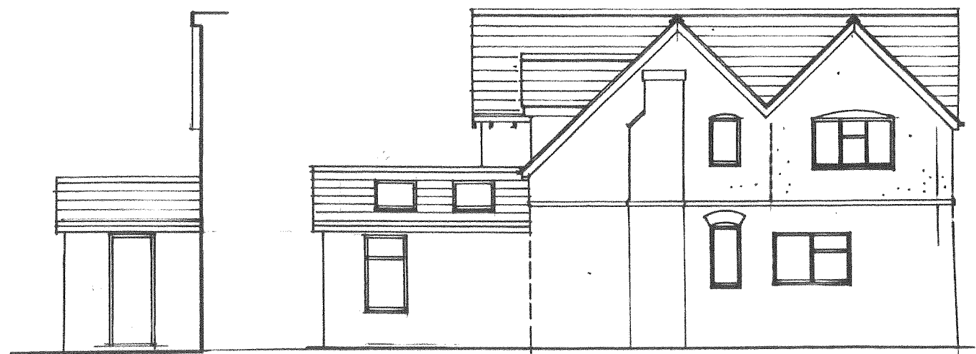
SIDE ELEVATION EAST PROPOSED.
