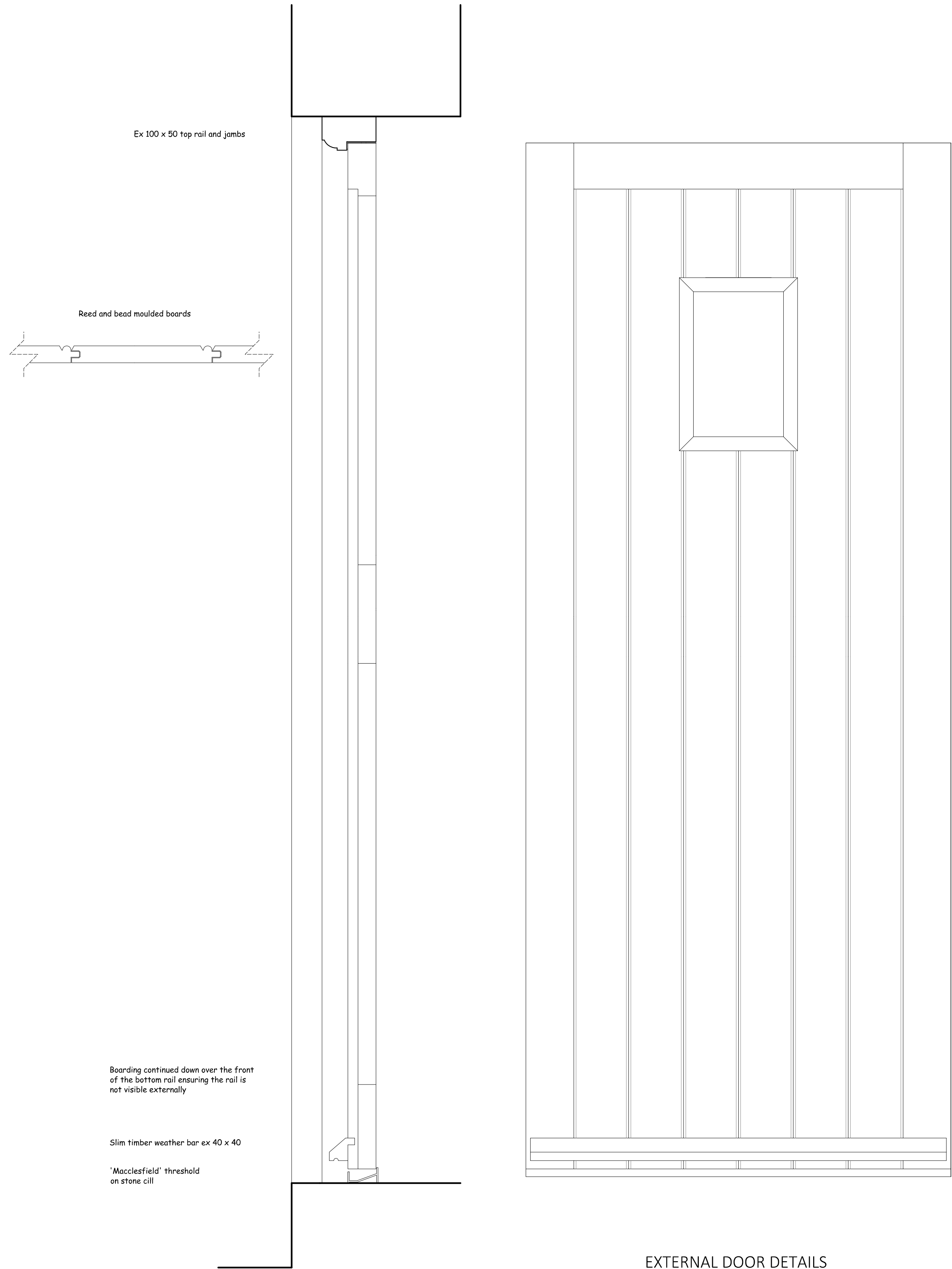
EXTERNAL DOOR DETAILS
