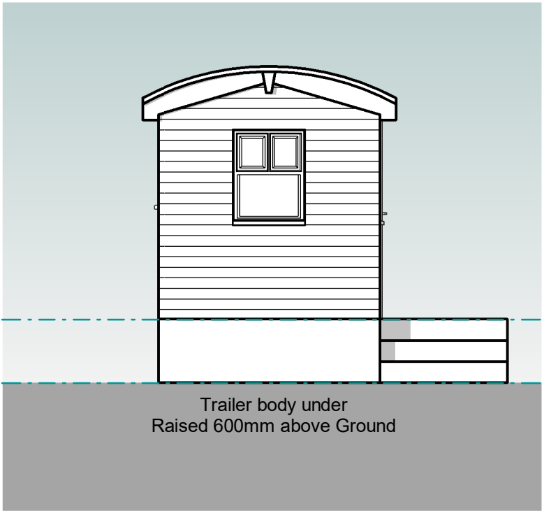
(03) West Elevation 1 : 50
