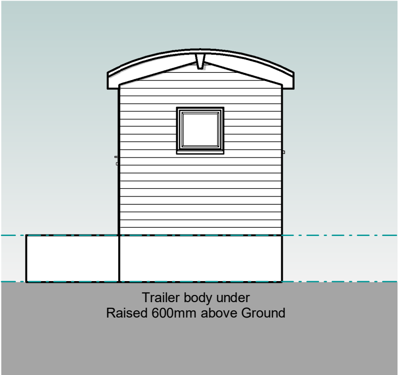
(03) East Elevation 1 : 50
