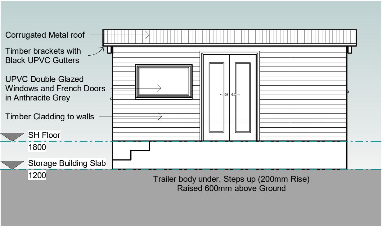
(03) South Elevation 1 : 50
