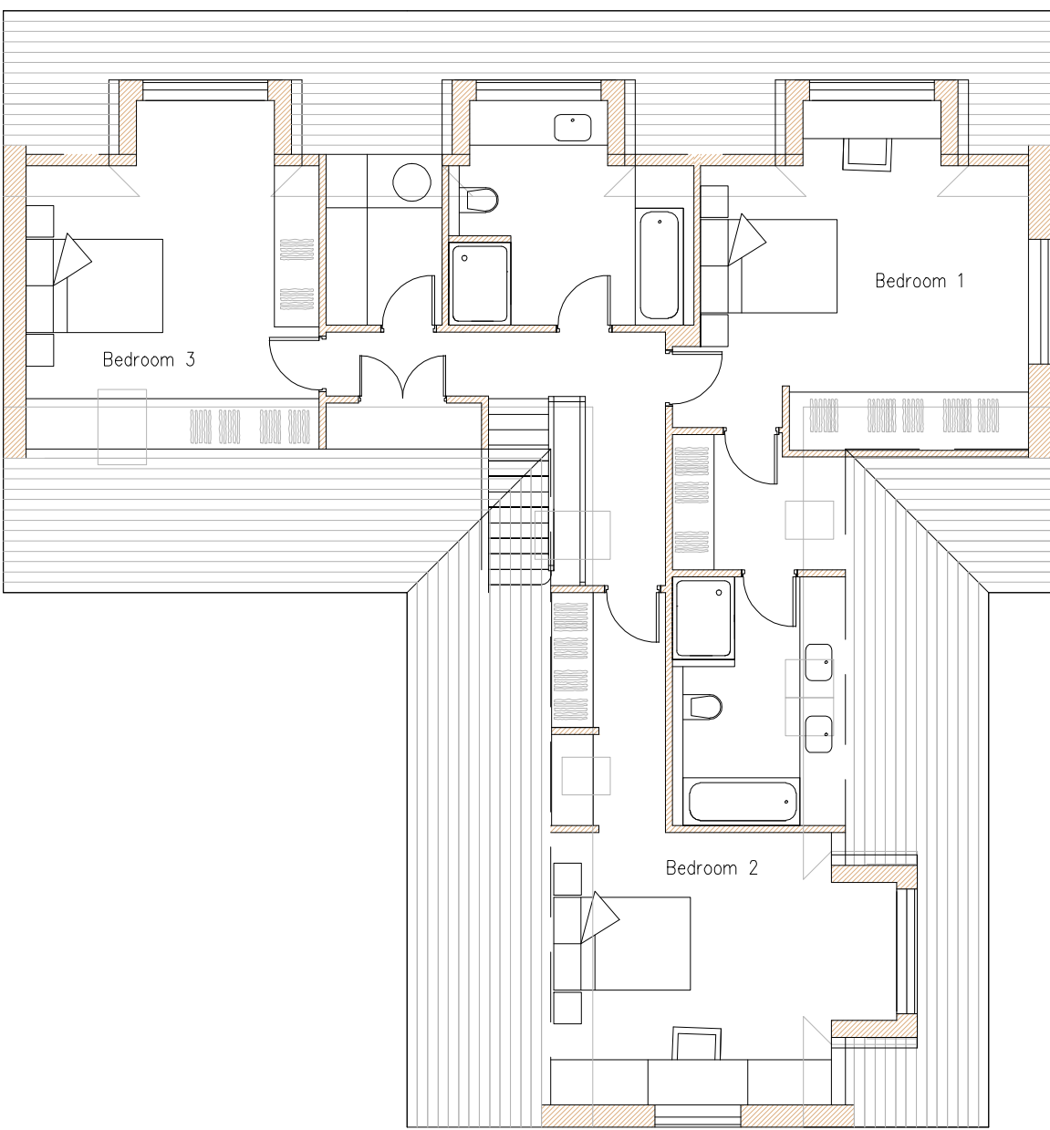
First Floor
