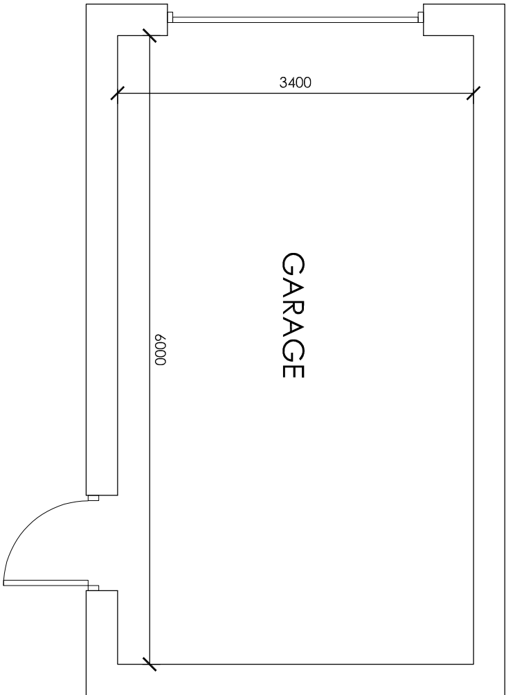
Floor Plan 1:50
